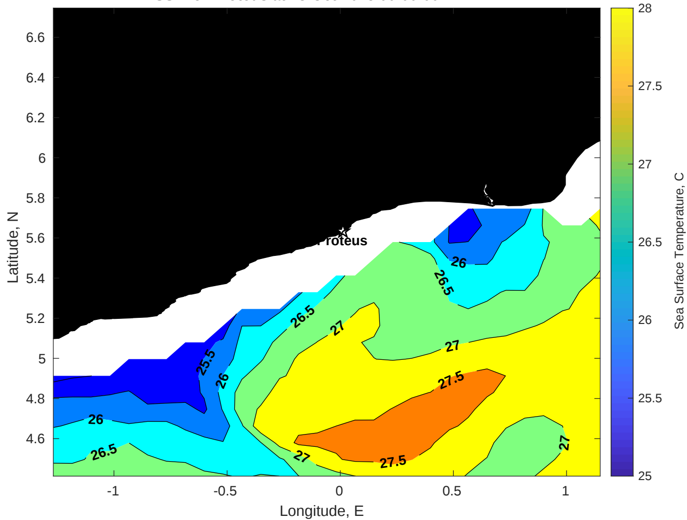
SST for Proteus at 13-Oct-2025 00:00:00
