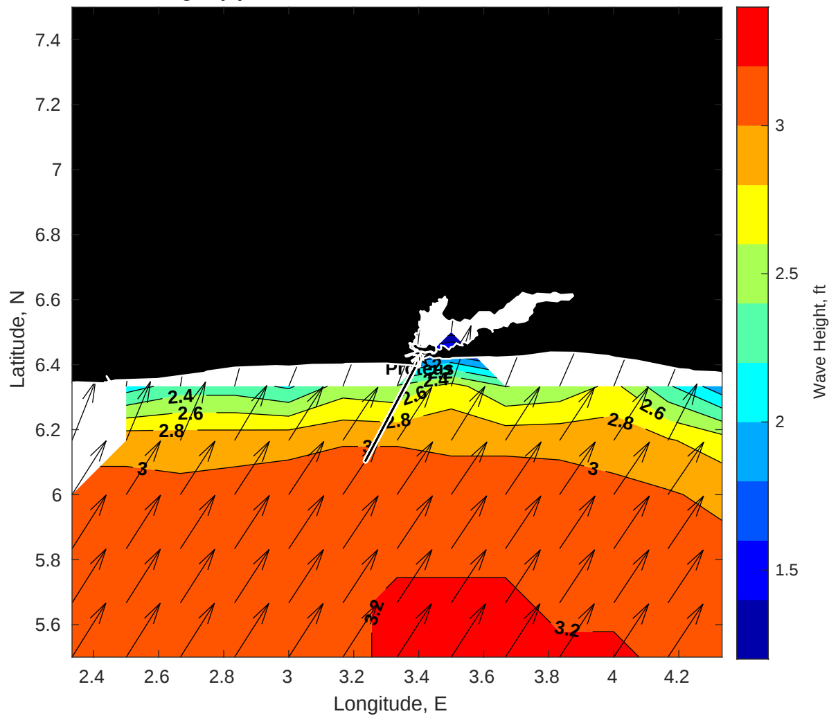
Wave Height (ft) for Proteus at 14-Oct-2025 09:00:00
