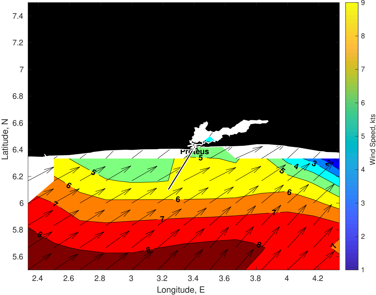
Winds (kts) for Proteus at 14-Oct-2025 09:00:00
