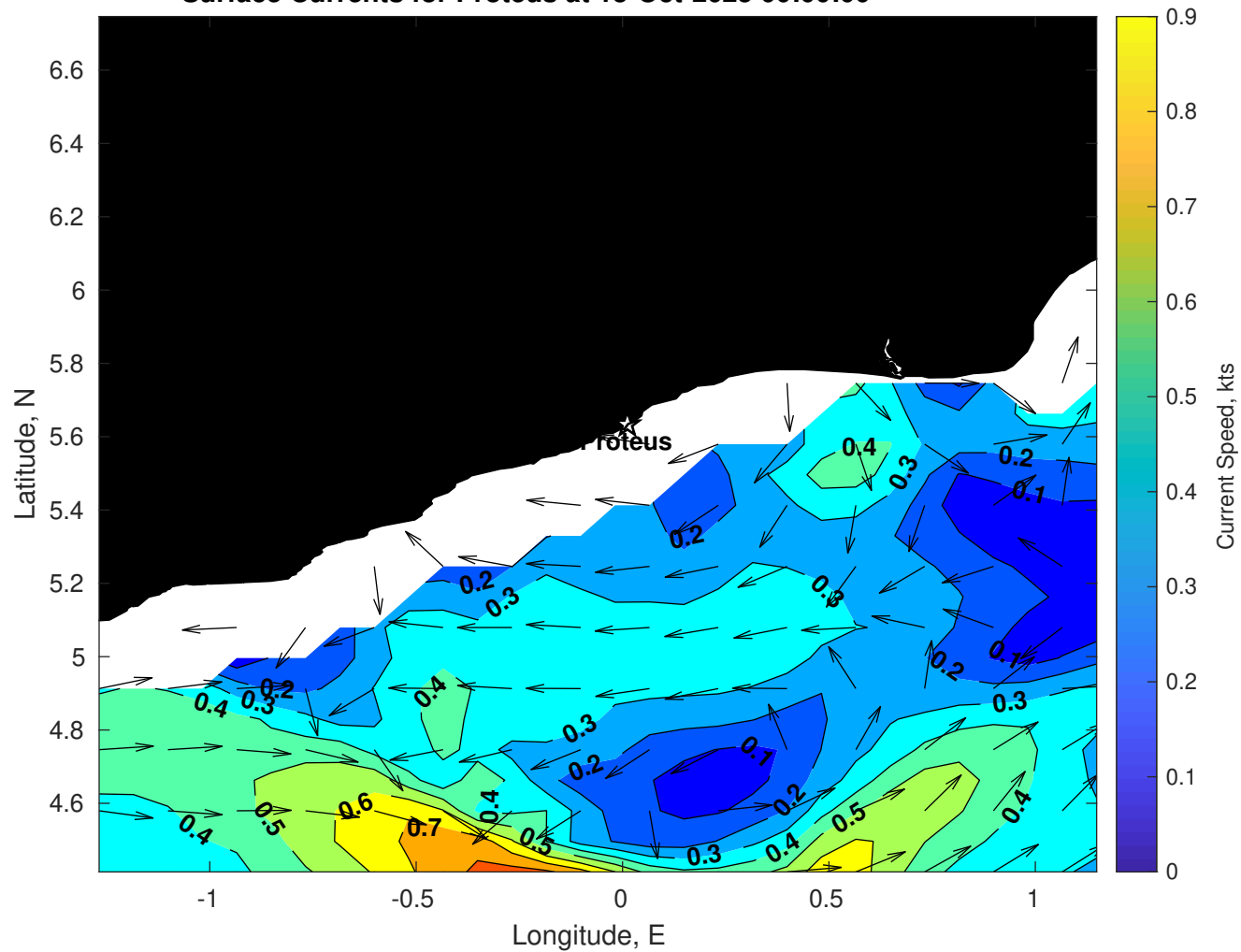
Surface Currents for Proteus at 13-Oct-2025 00:00:00
