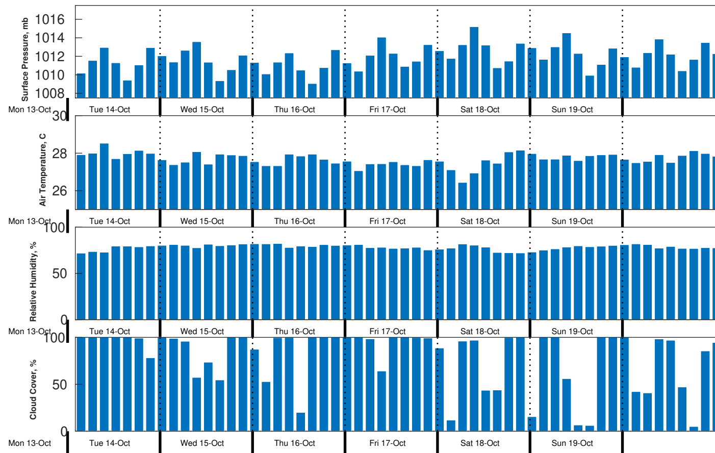
Met Forecast for Proteus from 14-Oct-2025 00:00:00 to 21-Oct-2025 00:00:00
