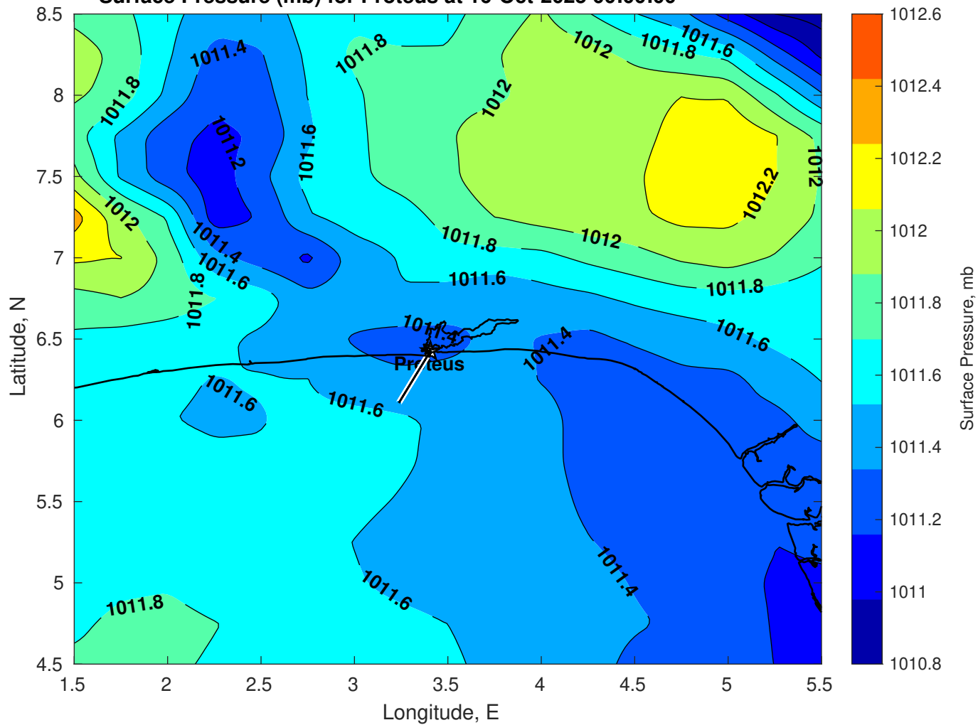
Surface Pressure (mb) for Proteus at 16-Oct-2025 00:00:00
