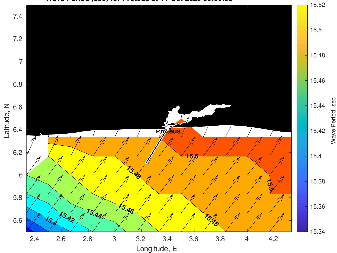
Wave Period (sec) for Proteus at 14-Oct-2025 09:00:00
