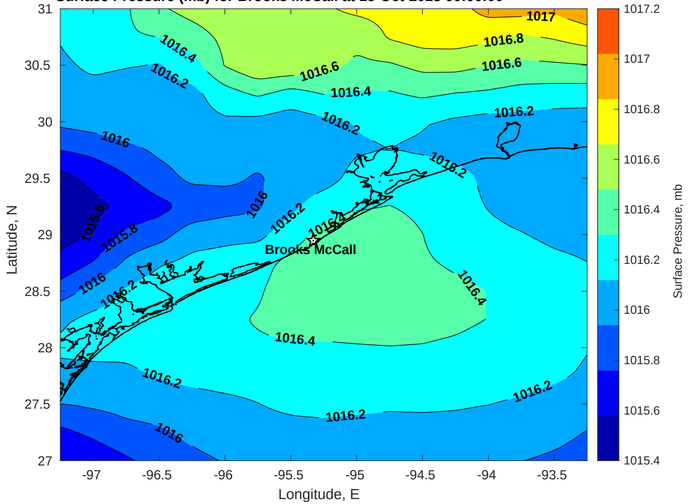
Surface Pressure (mb) for Brooks McCall at 15-Oct-2025 00:00:00
