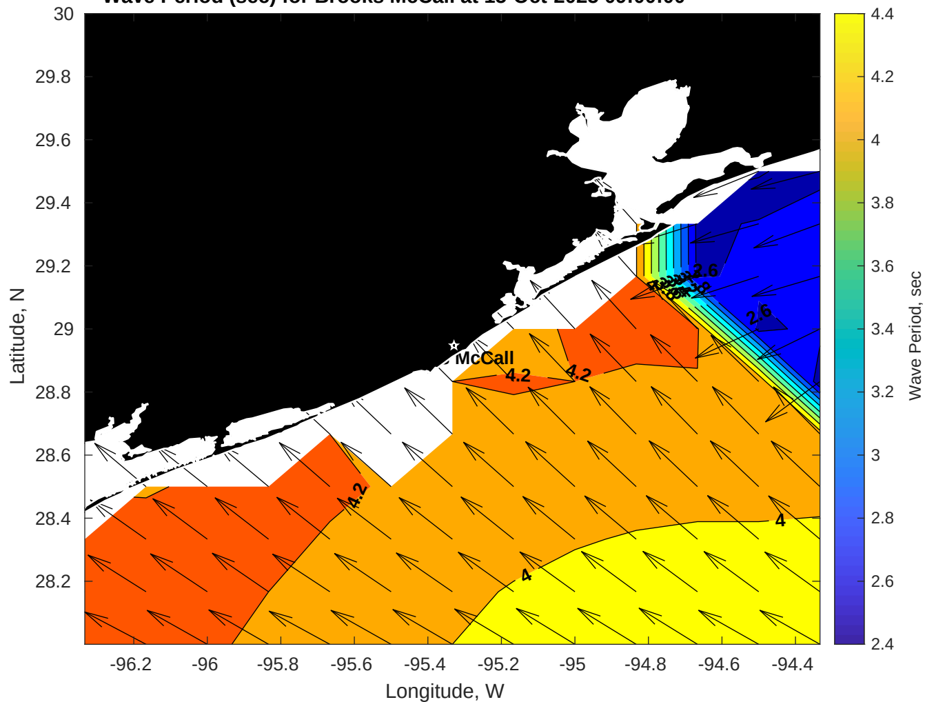
Wave Period (sec) for Brooks McCall at 15-Oct-2025 09:00:00
