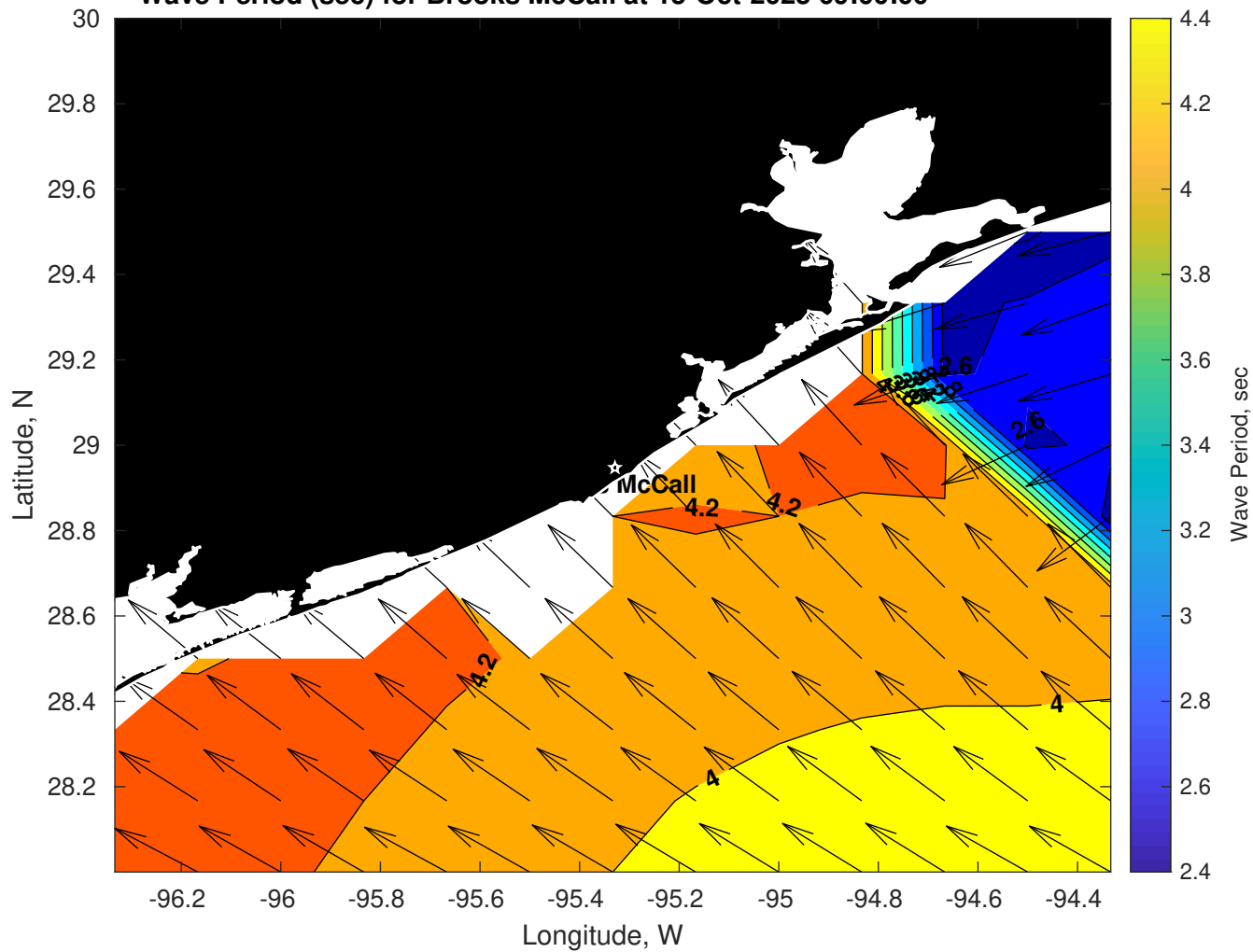
Wave Period (sec) for Brooks McCall at 15-Oct-2025 09:00:00
