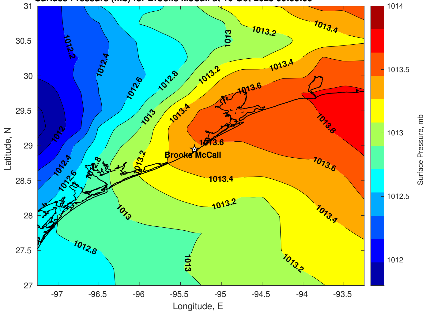
Surface Pressure (mb) for Brooks McCall at 16-Oct-2025 00:00:00
