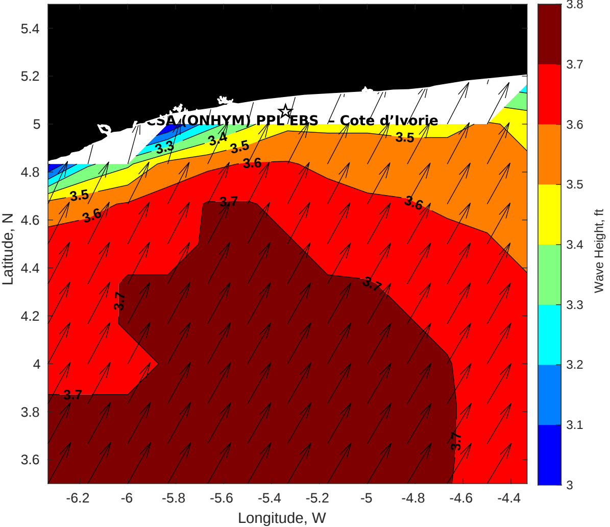
Wave Height (ft) for CSA (ONHYM) PPL EBS - Cote d'Ivoire at 15-Oct-2025 09:00:00
