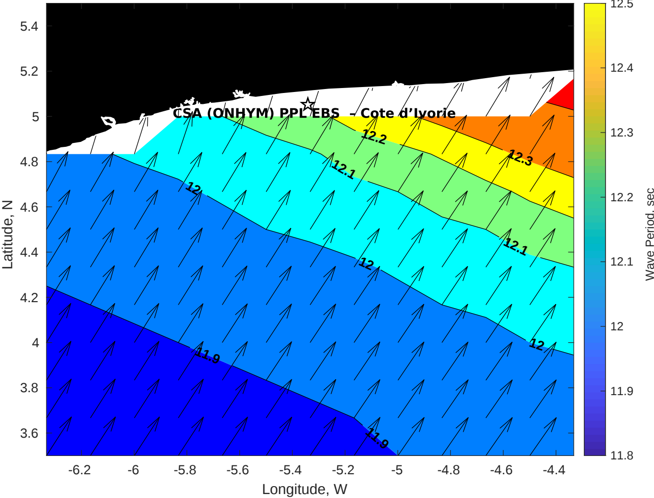
Wave Period (sec) for CSA (ONHYM) PPL EBS - Cote d'Ivoire at 15-Oct-2025 09:00:00
