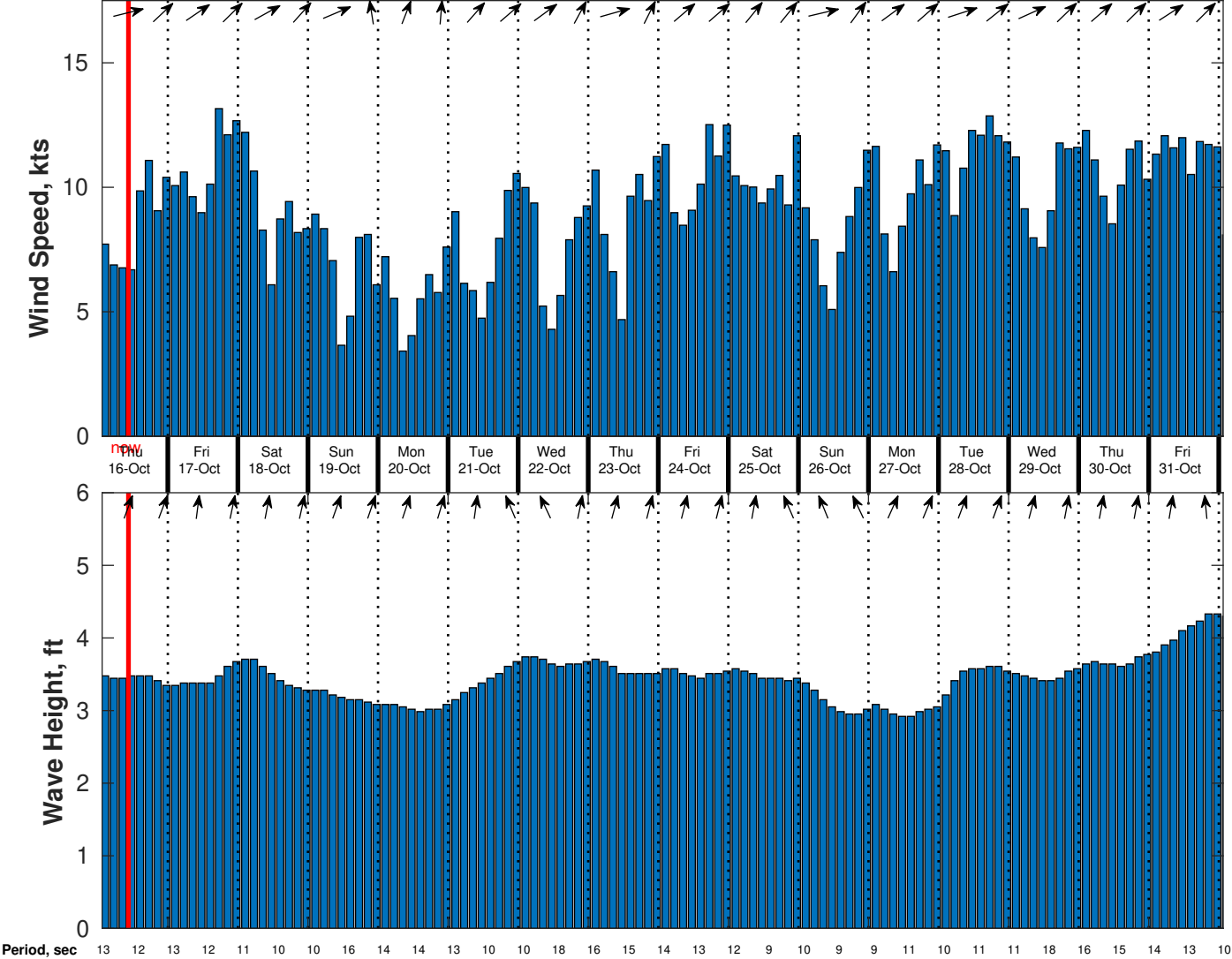
Wind & Wave Forecast for CSA (ONHYM) PPL EBS - Cote d'Ivoire from 15-Oct-2025 01:00:00 to 31-Oct-2025 01:00:00
