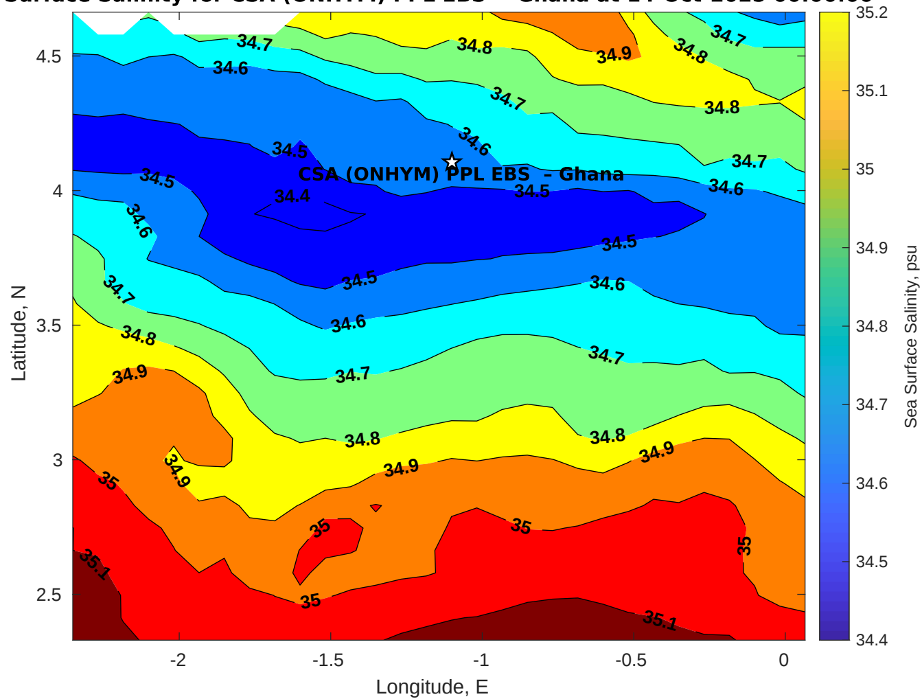
Surface Salinity for CSA (ONHYM) PPL EBS - Ghana at 14-Oct-2025 00:00:00
