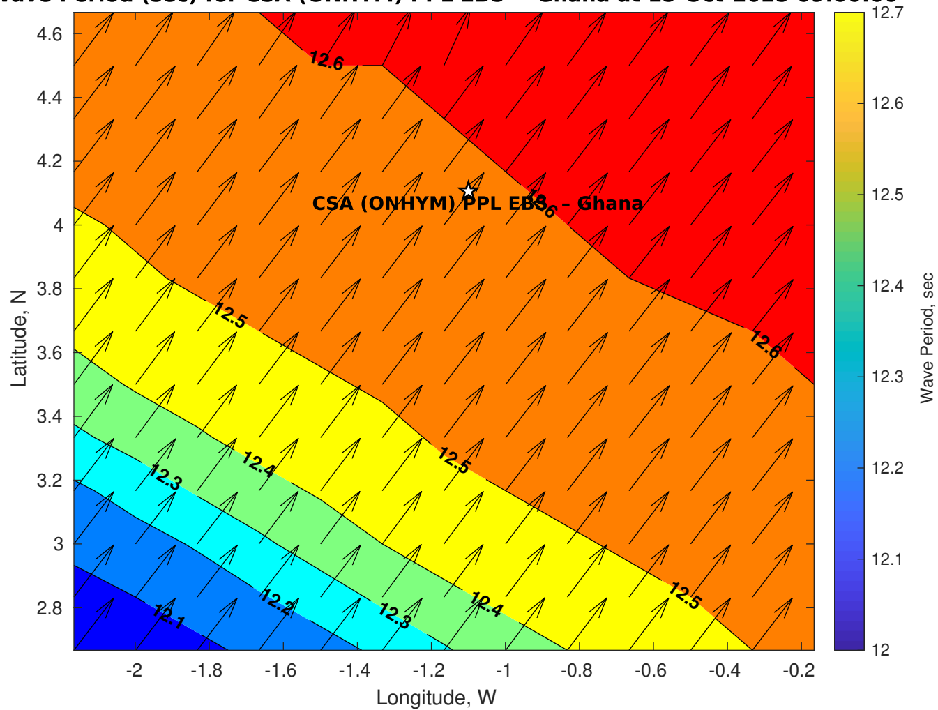
Wave Period (sec) for CSA (ONHYM) PPL EBS - Ghana at 15-Oct-2025 09:00:00
