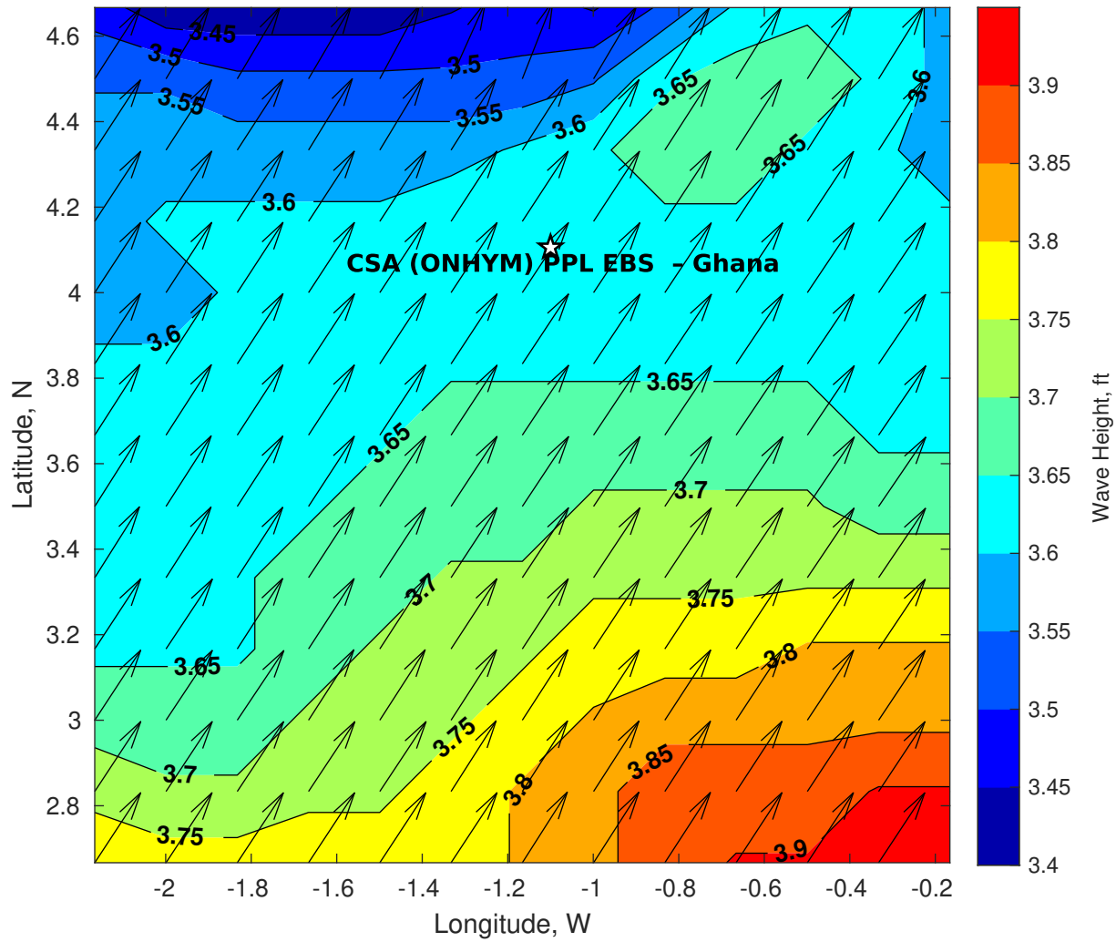
Wave Height (ft) for CSA (ONHYM) PPL EBS - Ghana at 15-Oct-2025 09:00:00
