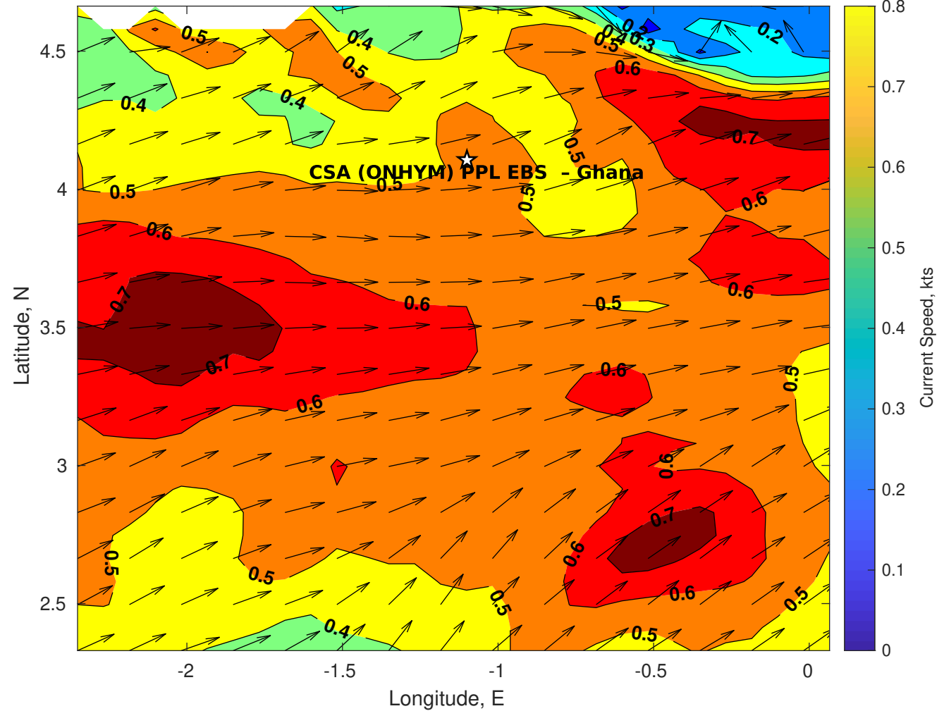
Surface Currents for CSA (ONHYM) PPL EBS - Ghana at 14-Oct-2025 00:00:00
