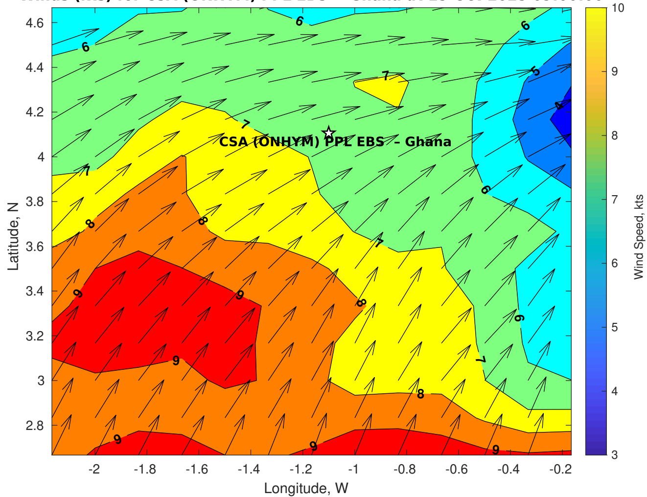
Winds (kts) for CSA (ONHYM) PPL EBS - Ghana at 15-Oct-2025 09:00:00
