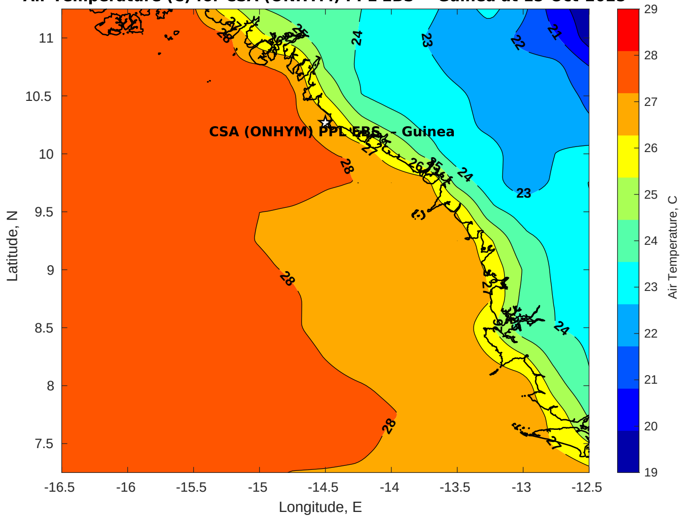
Air Temperature (C) for CSA (ONHYM) PPL EBS - Guinea at 15-Oct-2025
