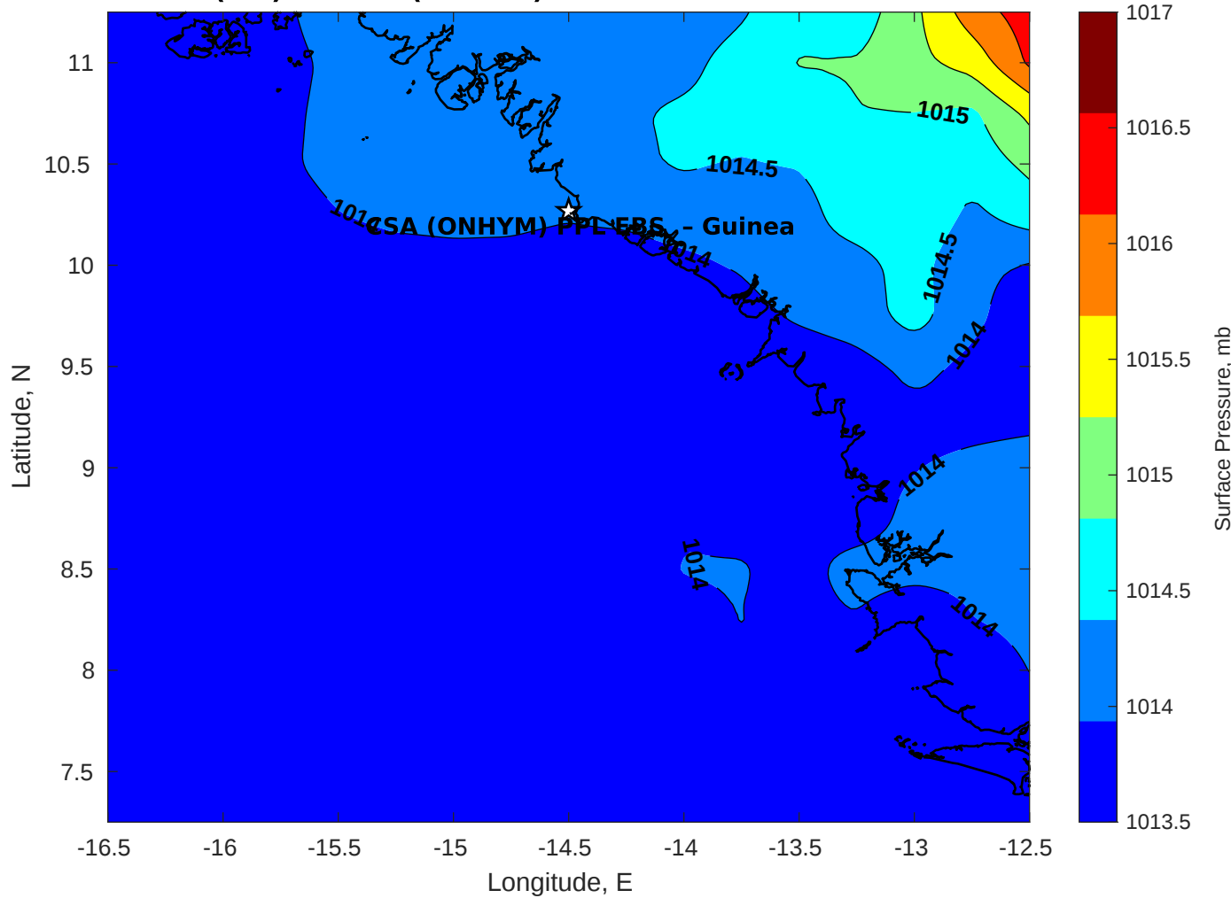
Surface Pressure (mb) for CSA (ONHYM) PPL EBS - Guinea at 15-Oct-2025 00:00:00
