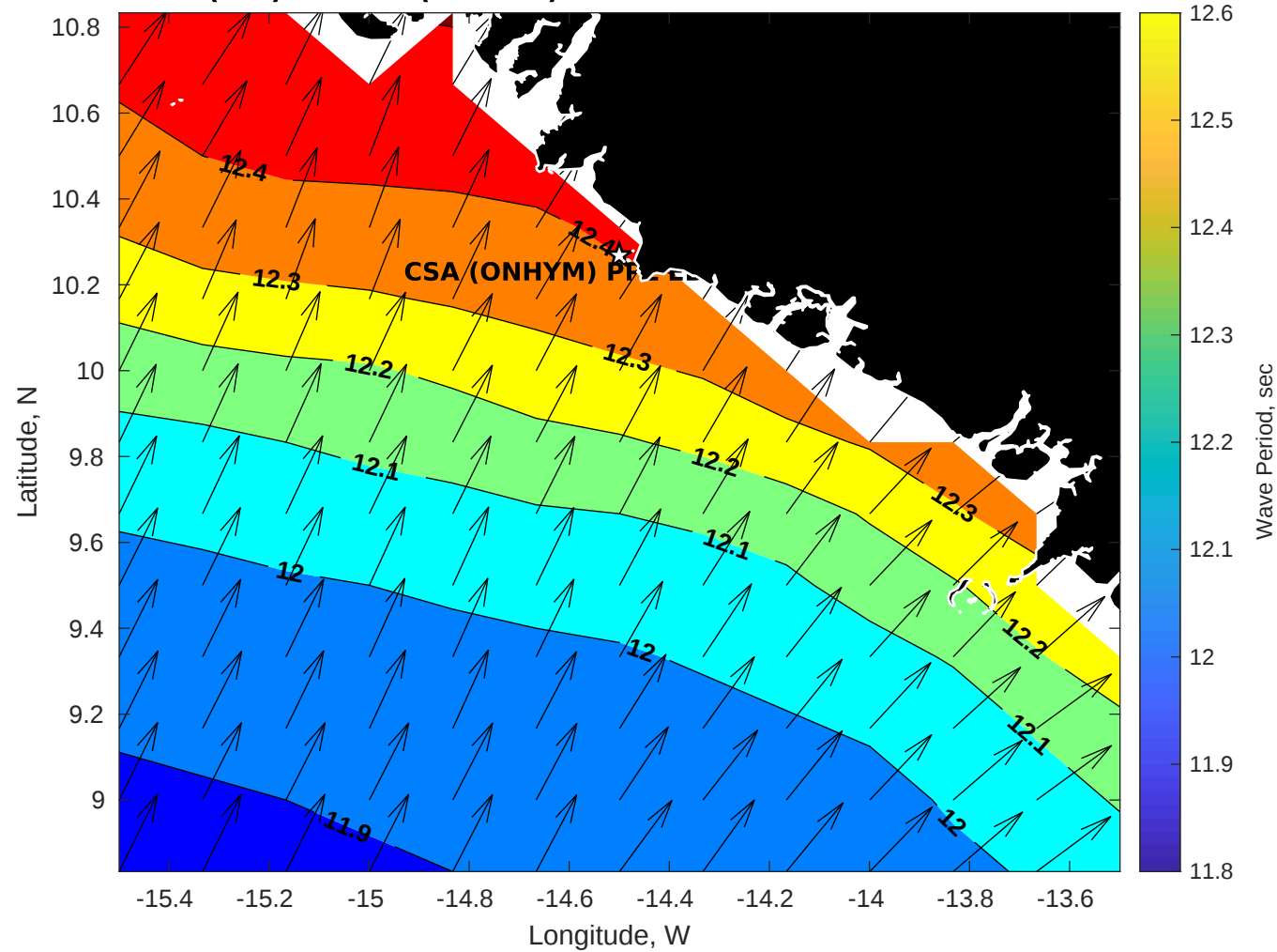
Wave Period (sec) for CSA (ONHYM) PPL EBS - Guinea at 15-Oct-2025 09:00:00
