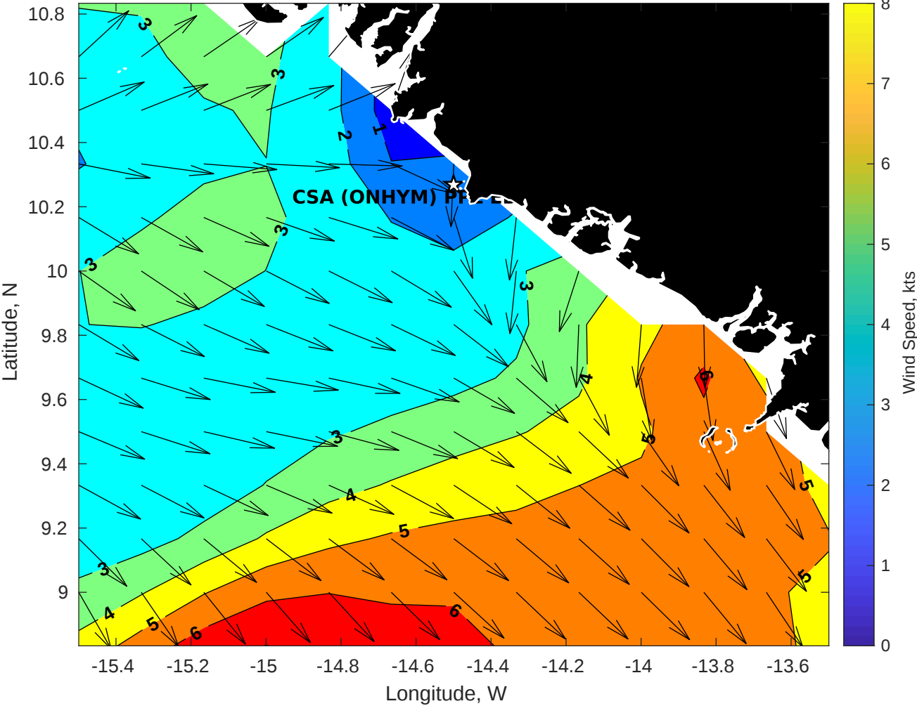
Winds (kts) for CSA (ONHYM) PPL EBS - Guinea at 15-Oct-2025 09:00:00
