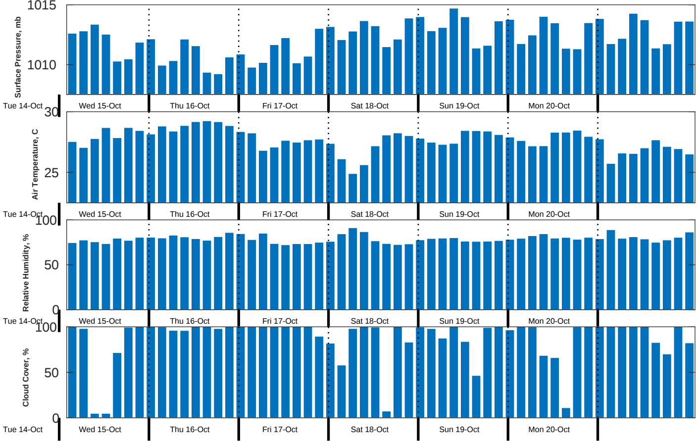
Met Forecast for CSA (ONHYM) PPL EBS - Guinea from 15-Oct-2025 00:00:00 to 22-Oct-2025 00:00:00
