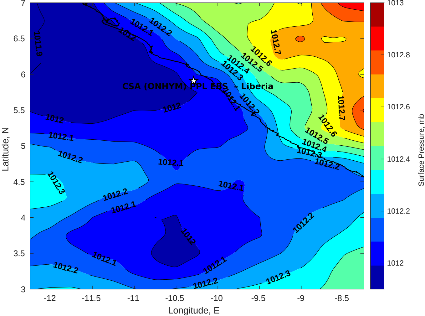
Surface Pressure (mb) for CSA (ONHYM) PPL EBS - Liberia at 17-Oct-2025 00:00:00
