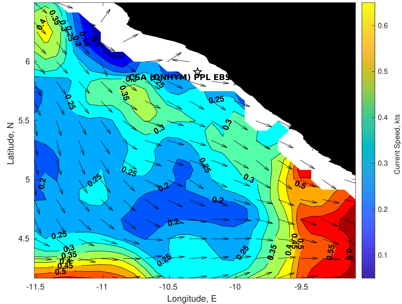
Surface Currents for CSA (ONHYM) PPL EBS - Liberia at 14-Oct-2025 00:00:00
