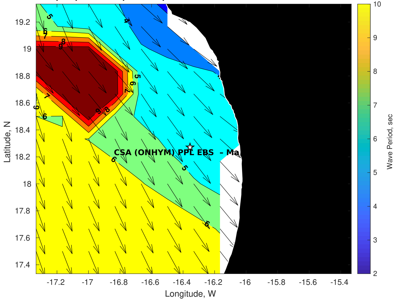
Wave Period (sec) for CSA (ONHYM) PPL EBS - Mauritania at 13-Oct-2025 21:00:00
