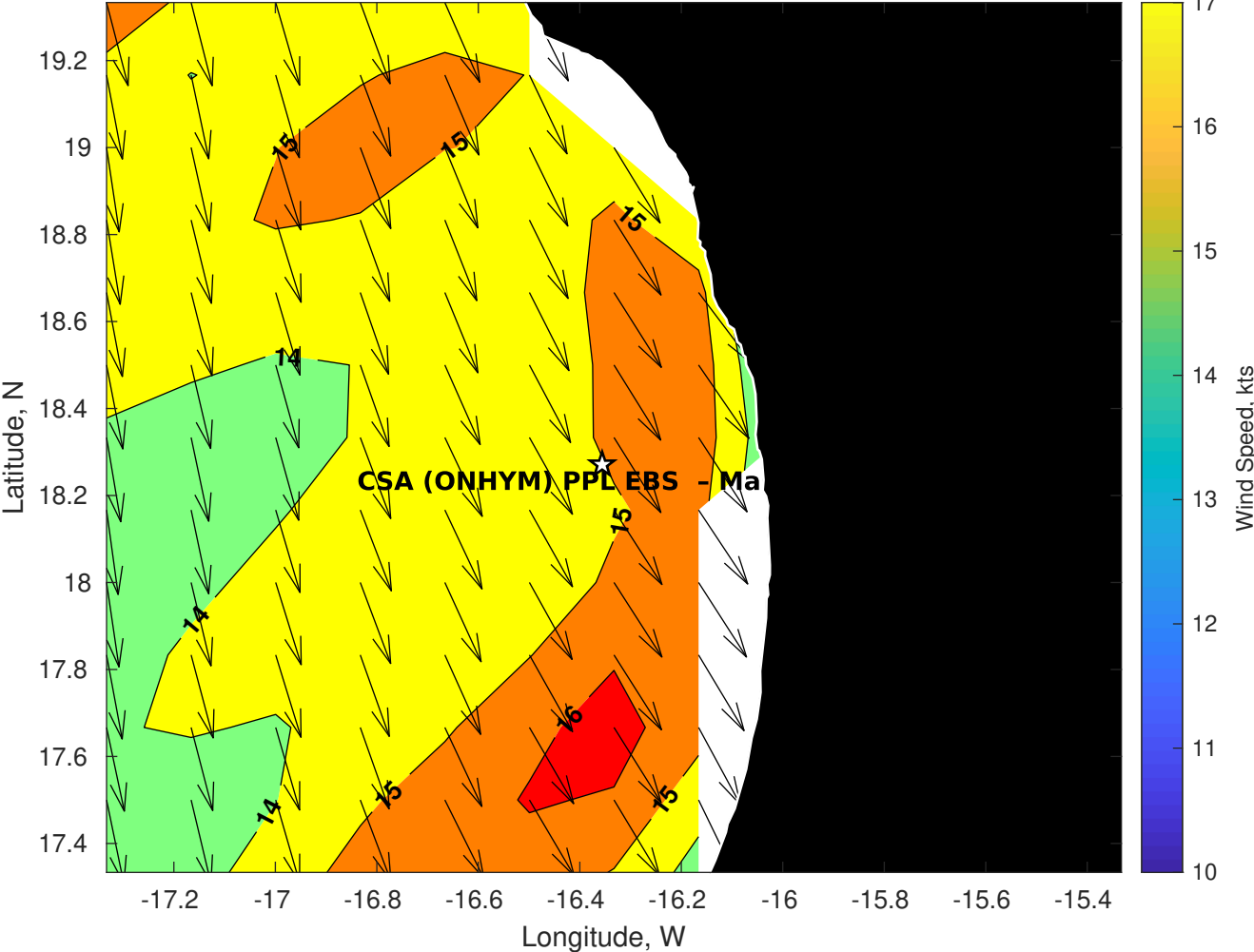
Winds (kts) for CSA (ONHYM) PPL EBS - Mauritania at 13-Oct-2025 21:00:00
