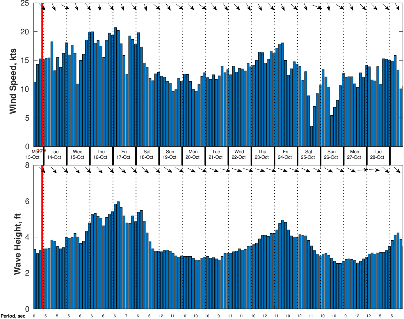
Wind & Wave Forecast for CSA (ONHYM) PPL EBS - Mauritania from 13-Oct-2025 13:00:00 to 29-Oct-2025 13:00:00
