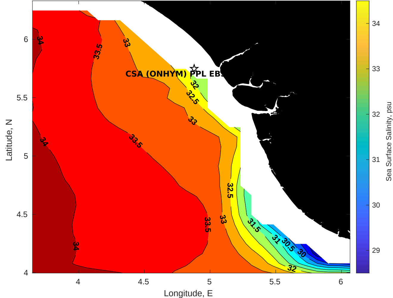
Surface Salinity for CSA (ONHYM) PPL EBS - Nigeria at 14-Oct-2025 00:00:00
