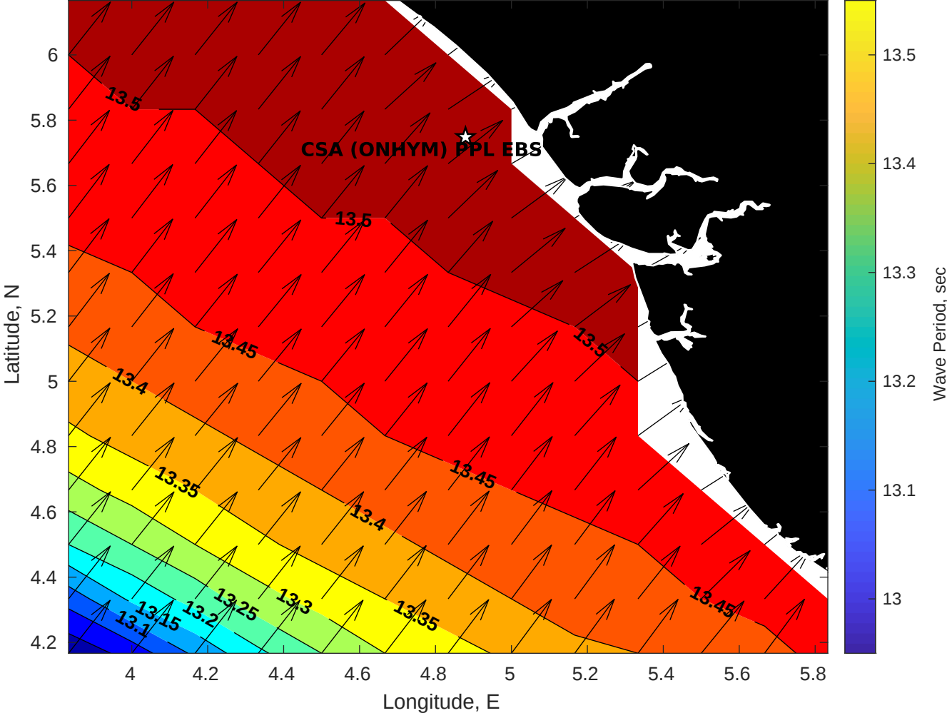
Wave Period (sec) for CSA (ONHYM) PPL EBS - Nigeria at 15-Oct-2025 09:00:00
