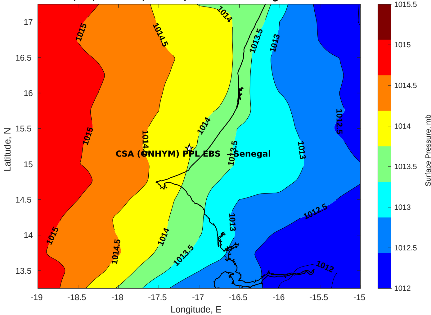
Surface Pressure (mb) for CSA (ONHYM) PPL EBS - Senegal at 15-Oct-2025 12:00:00
