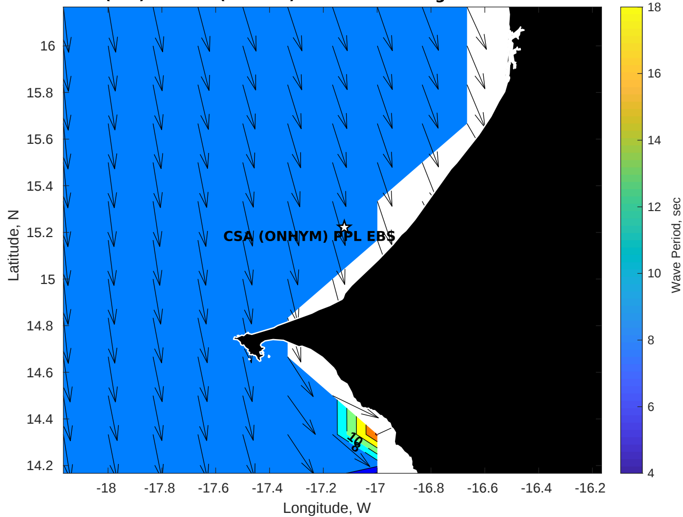
Wave Period (sec) for CSA (ONHYM) PPL EBS - Senegal at 13-Oct-2025 21:00:00
