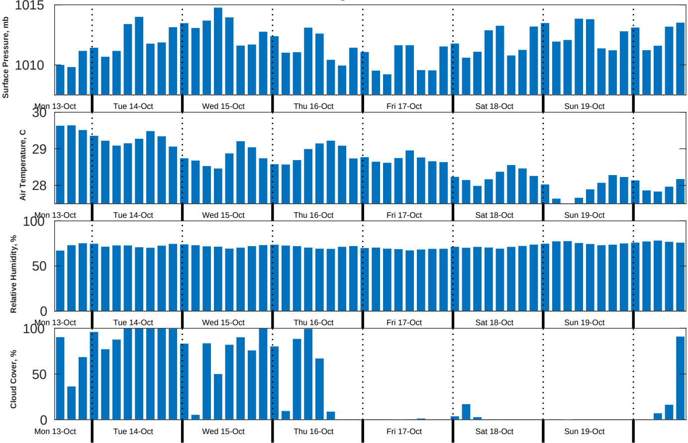
Met Forecast for CSA (ONHYM) PPL EBS - Senegal from 13-Oct-2025 12:00:00 to 20-Oct-2025 12:00:00
