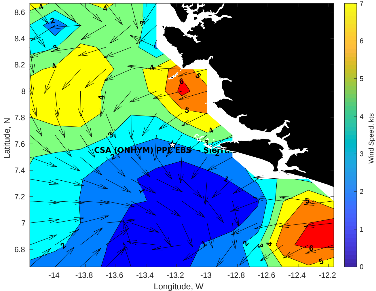
Winds (kts) for CSA (ONHYM) PPL EBS - Sierra Leone at 15-Oct-2025 09:00:00
