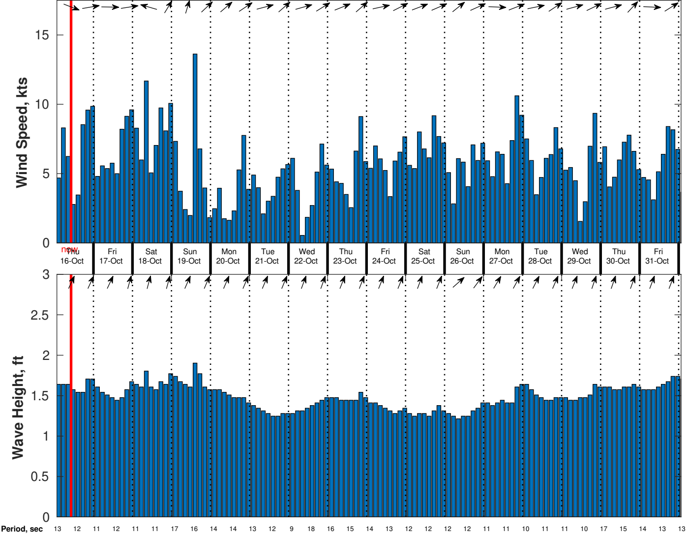
Wind & Wave Forecast for CSA (ONHYM) PPL EBS - Sierra Leone from 15-Oct-2025 01:00:00 to 31-Oct-2025 01:00:00
