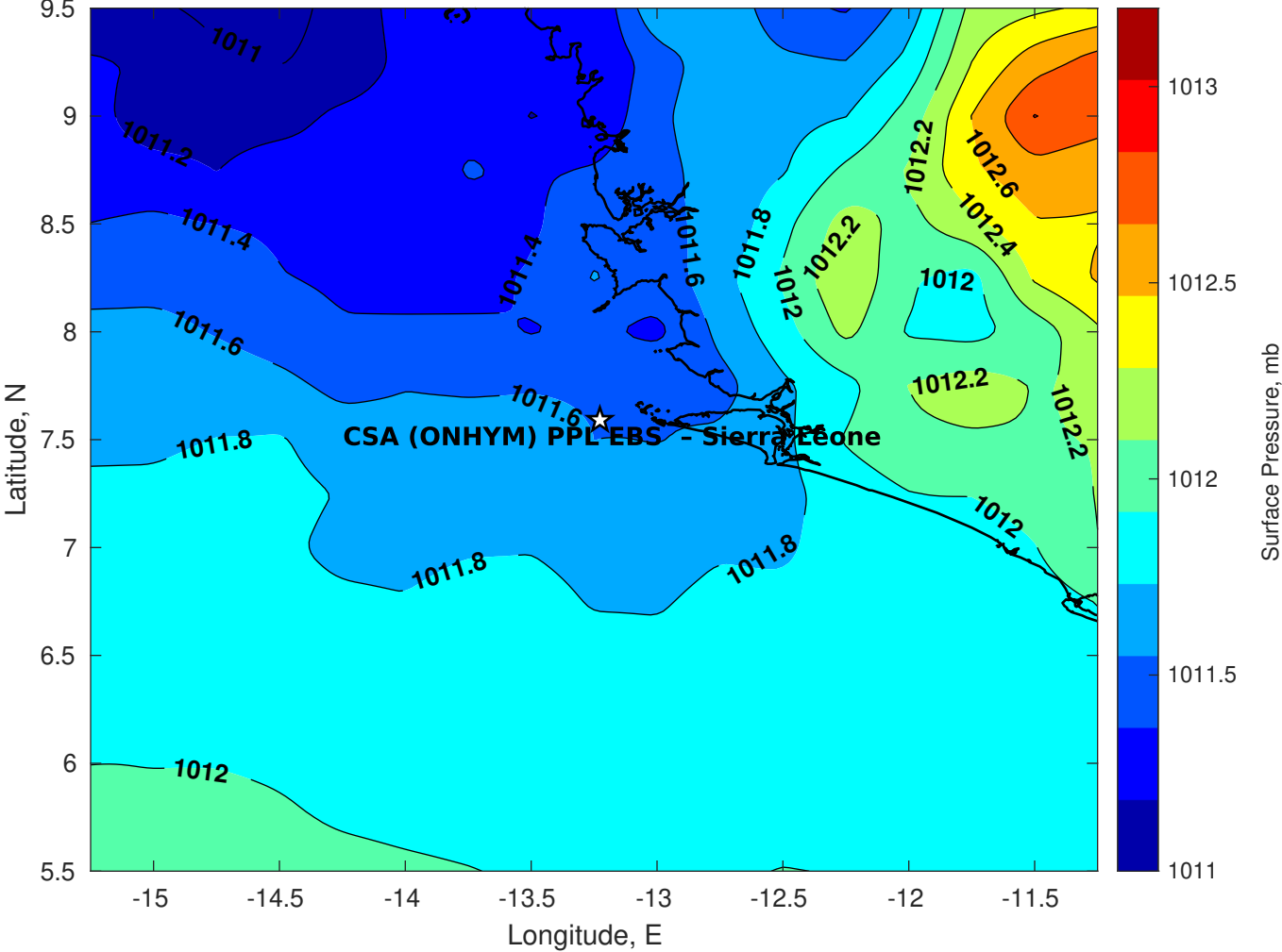
Surface Pressure (mb) for CSA (ONHYM) PPL EBS - Sierra Leone at 17-Oct-2025 00:00:00
