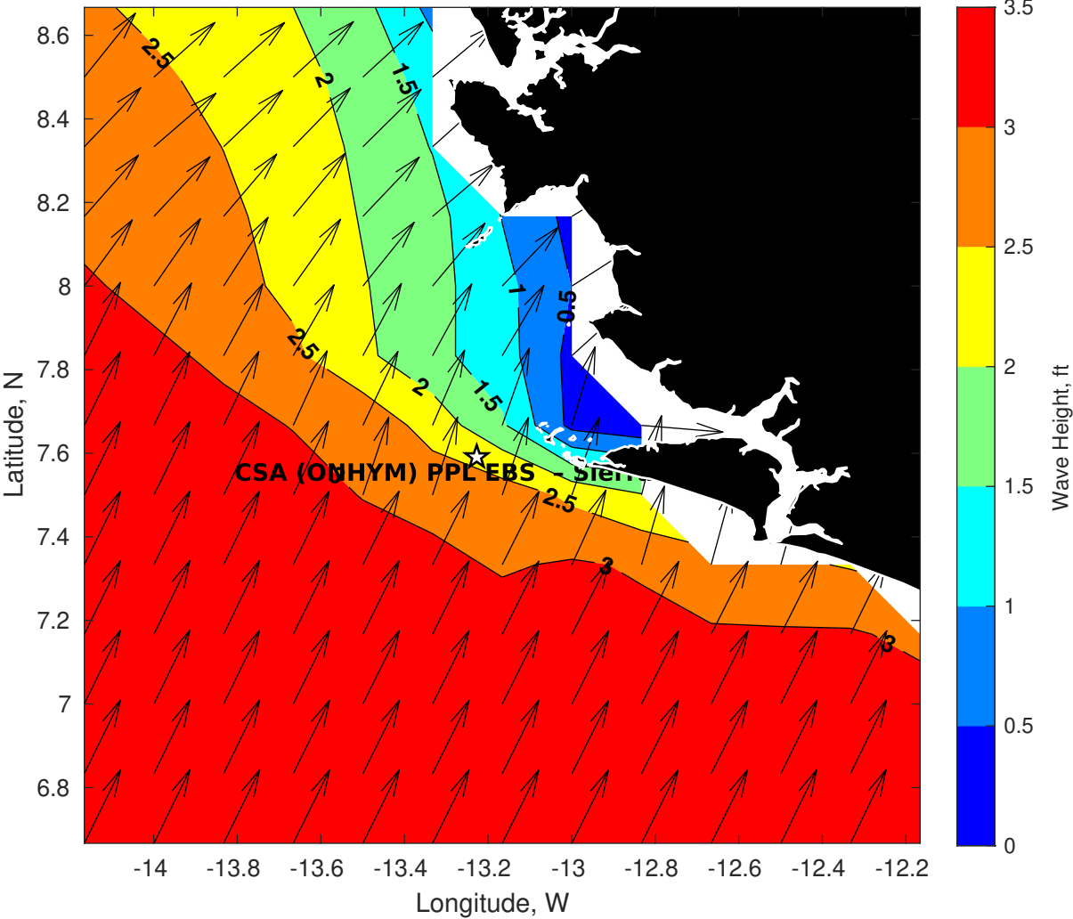
Wave Height (ft) for CSA (ONHYM) PPL EBS - Sierra Leone at 15-Oct-2025 09:00:00
