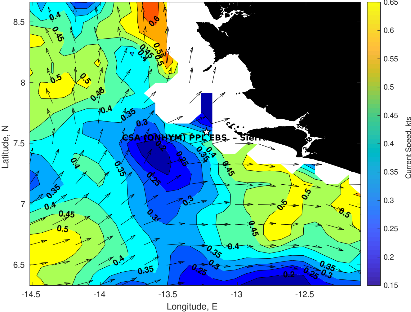
Surface Currents for CSA (ONHYM) PPL EBS - Sierra Leone at 14-Oct-2025 00:00:00
