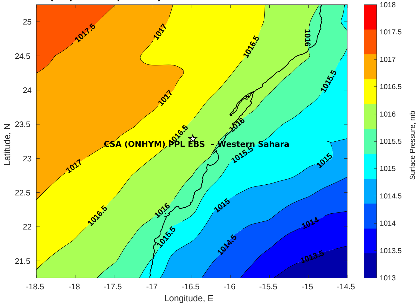
Surface Pressure (mb) for CSA (ONHYM) PPL EBS - Western Sahara at 15-Oct-2025 12:00:00
