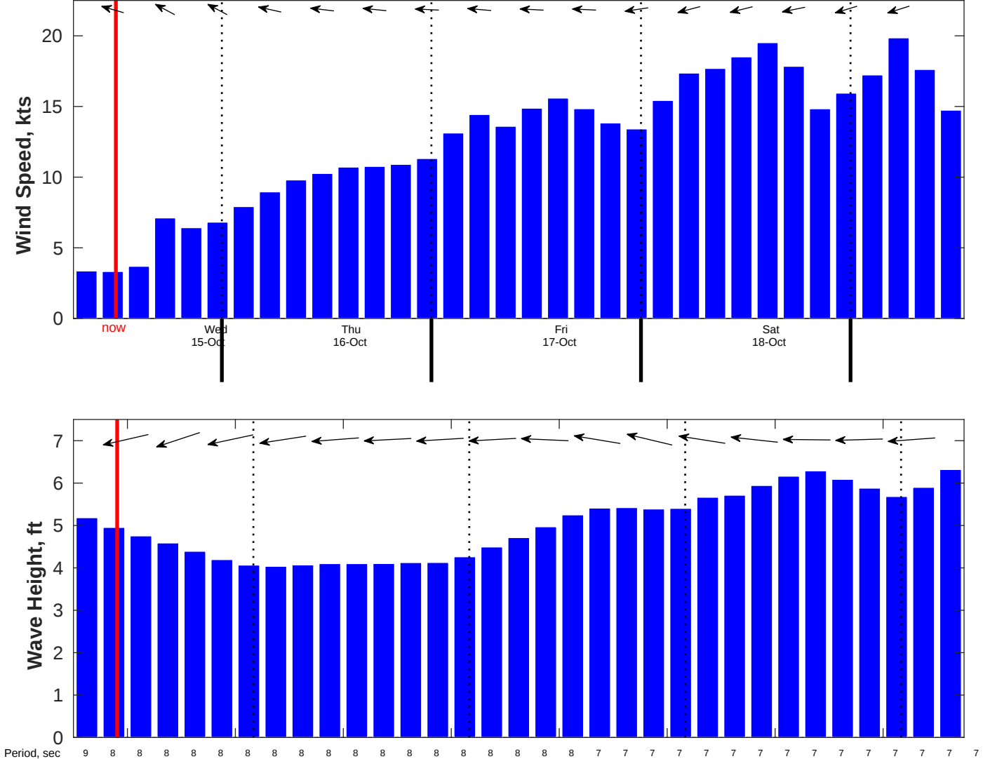
Wind & Wave Forecast for Gyre Passage: Dakar to Trinidad from 15-Oct-2025 06:00:00 to 19-Oct-2025 09:00:00
