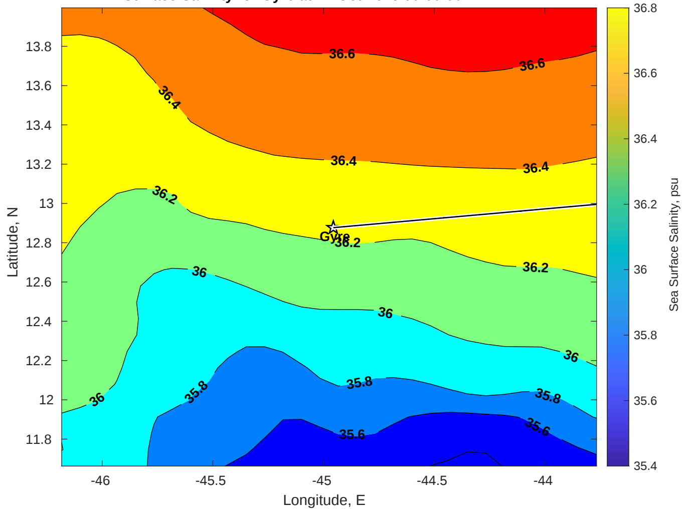
Surface Salinity for Gyre at 14-Oct-2025 00:00:00
