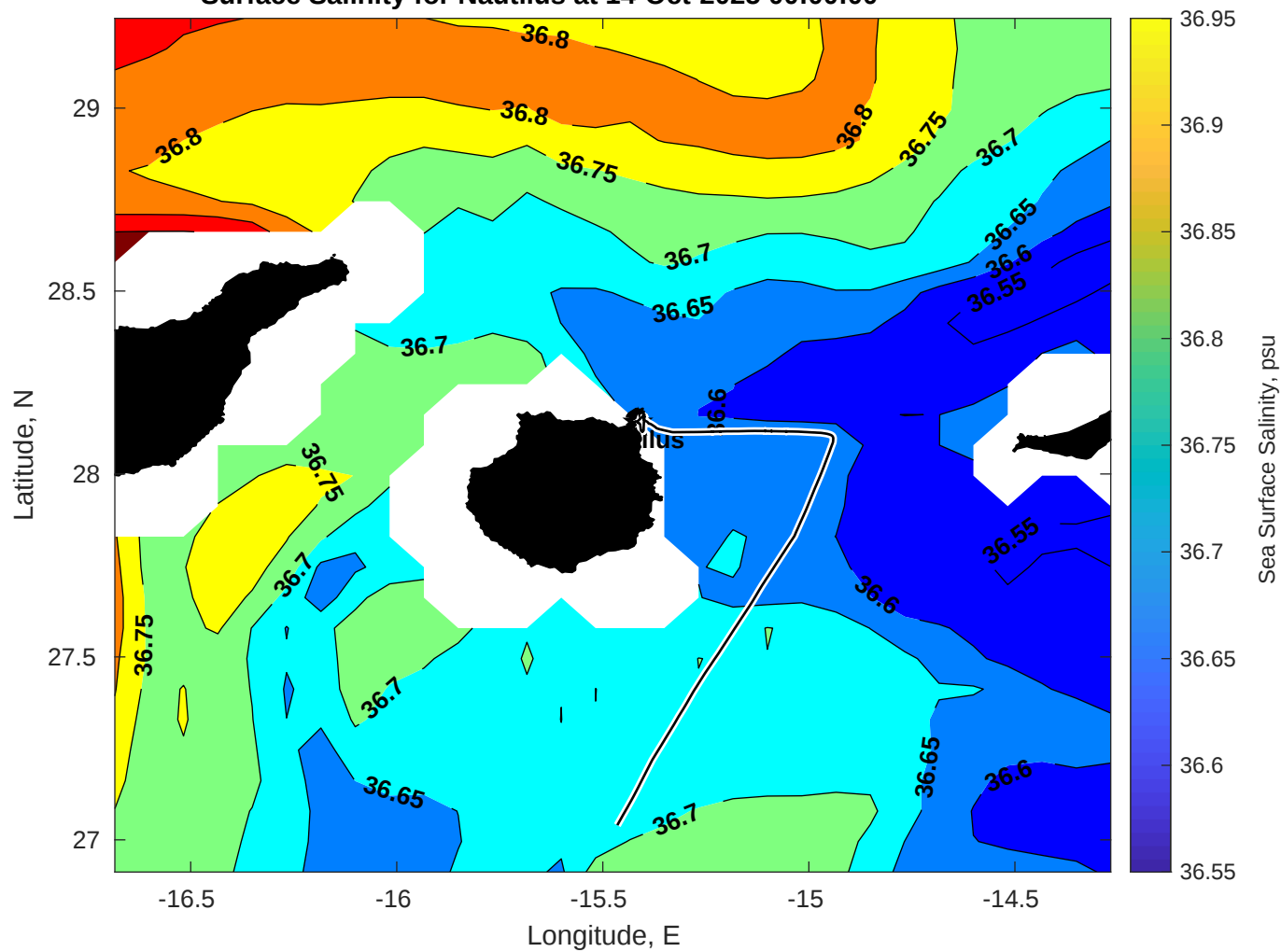
Surface Salinity for Nautilus at 14-Oct-2025 00:00:00
