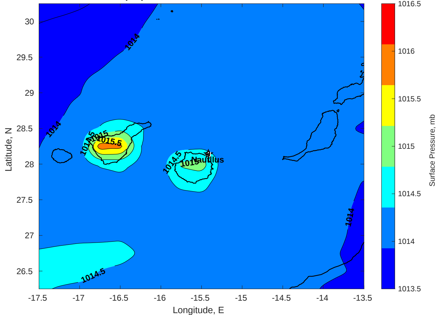
Surface Pressure (mb) for Nautilus at 17-Oct-2025 00:00:00
