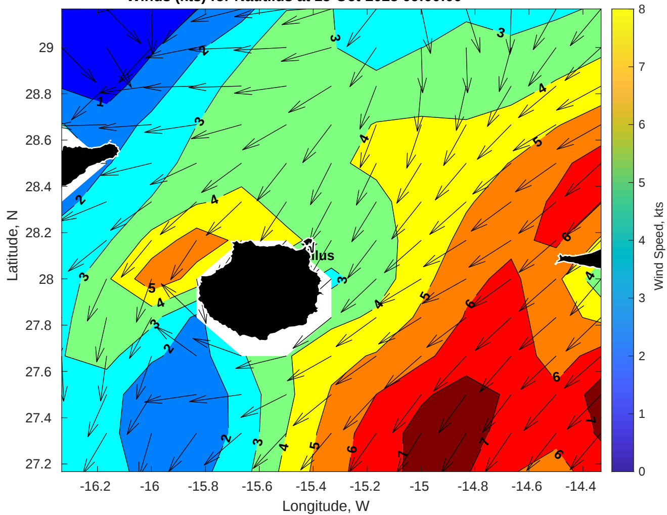
Winds (kts) for Nautilus at 15-Oct-2025 09:00:00
