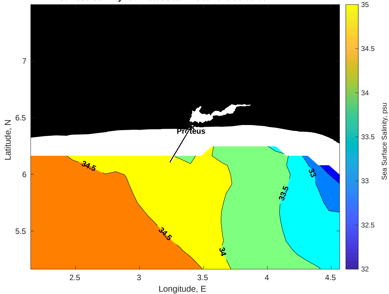
Surface Salinity for Proteus at 14-Oct-2025 00:00:00
