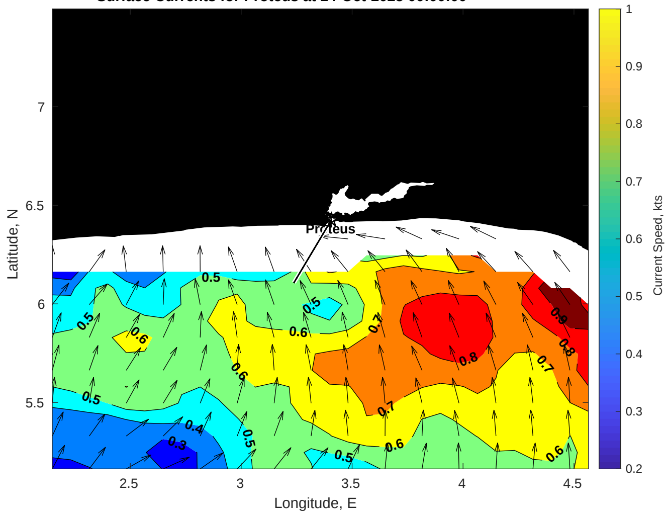
Surface Currents for Proteus at 14-Oct-2025 00:00:00
