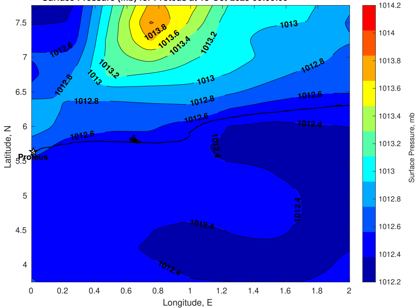
Surface Pressure (mb) for Proteus at 15-Oct-2025 00:00:00
