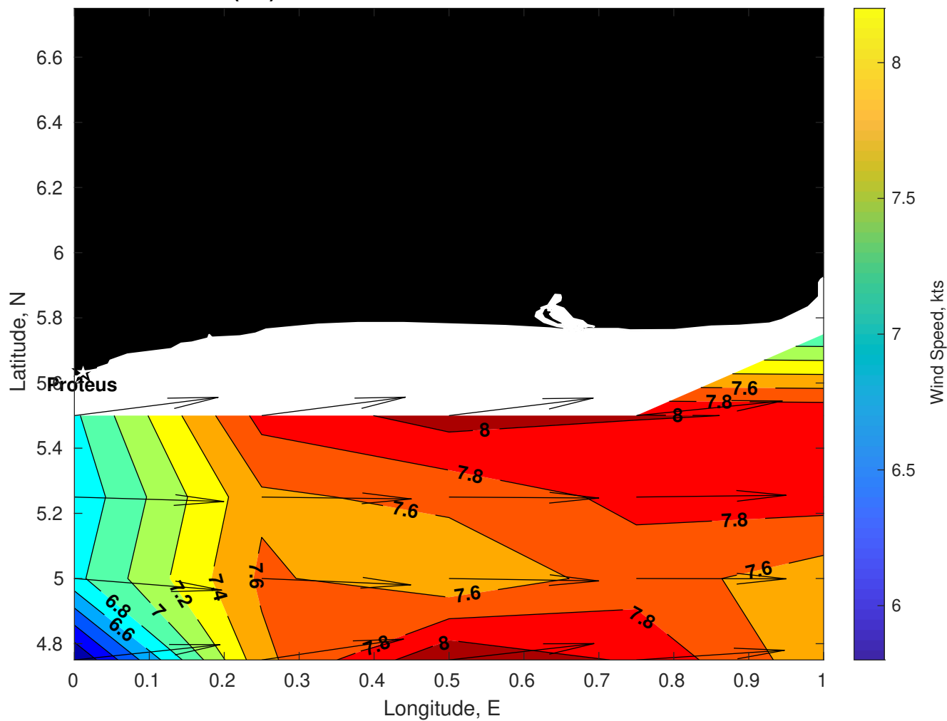
Winds (kts) for Proteus at 15-Oct-2025 09:00:00
