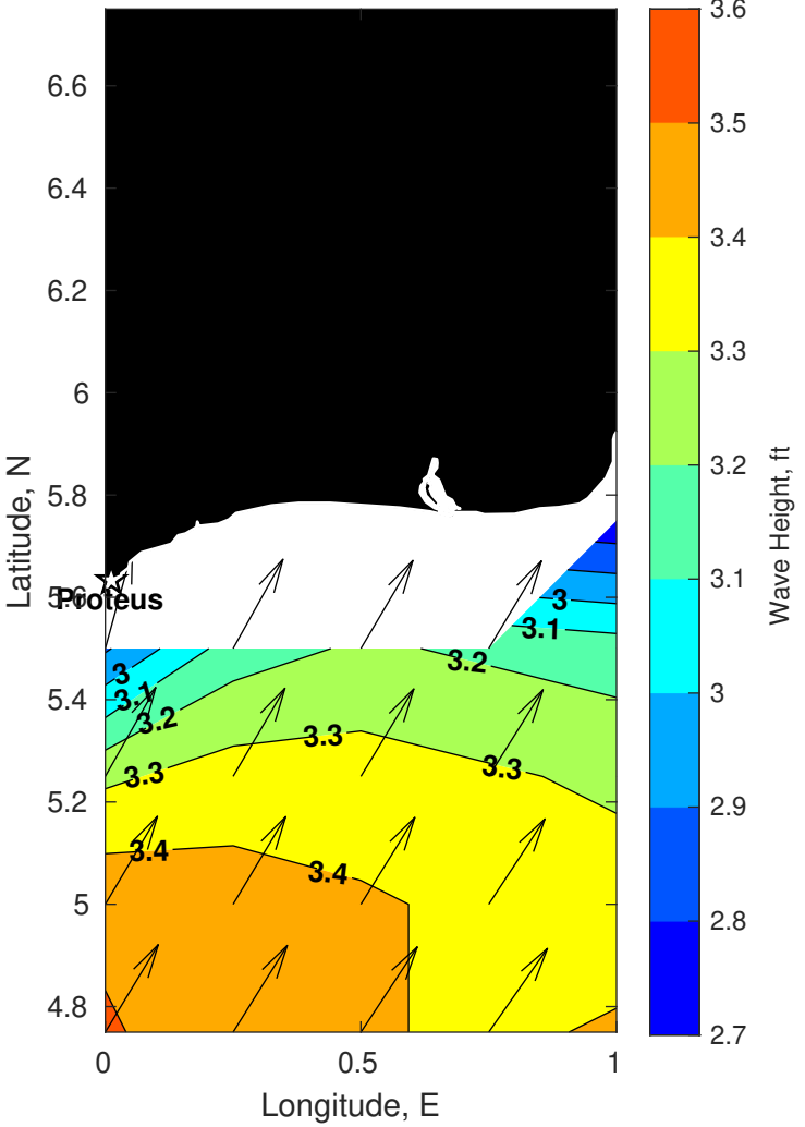
Wave Height (ft) for Proteus at 15-Oct-2025 09:00:00
