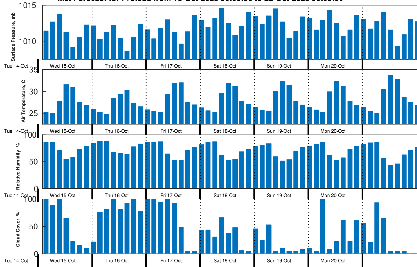
Met Forecast for Proteus from 15-Oct-2025 00:00:00 to 22-Oct-2025 00:00:00
