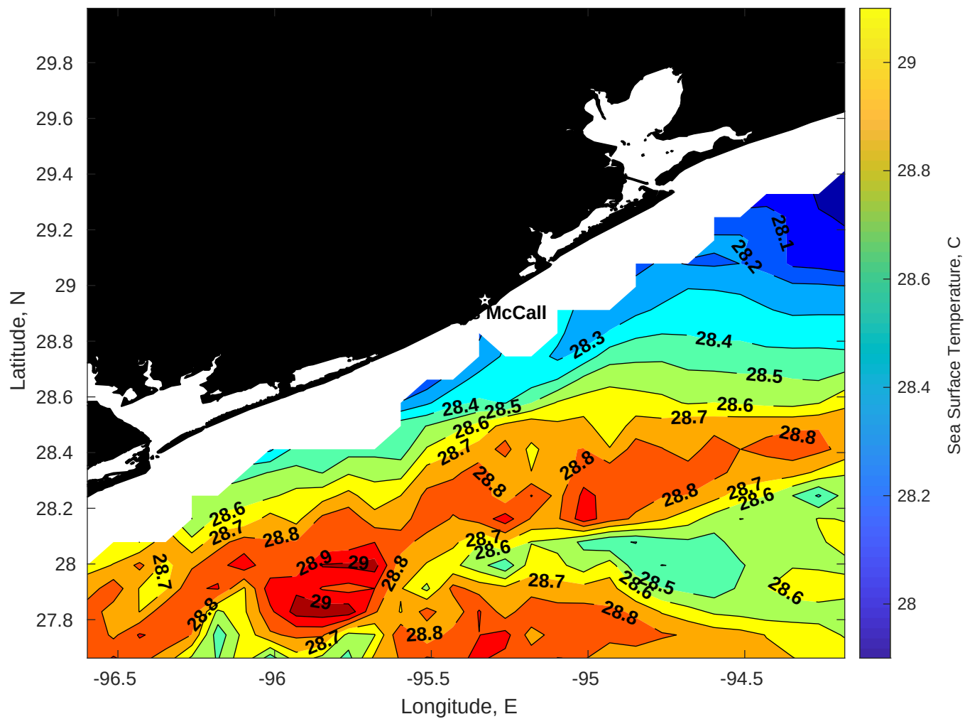
SST for Brooks McCall at 15-Oct-2025 00:00:00
