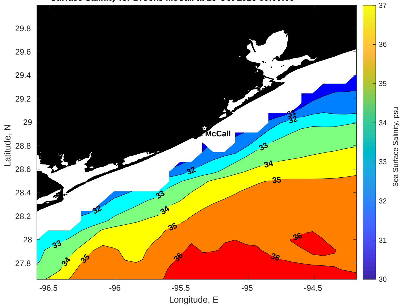
Surface Salinity for Brooks McCall at 15-Oct-2025 00:00:00
