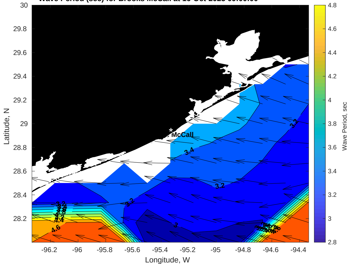
Wave Period (sec) for Brooks McCall at 16-Oct-2025 09:00:00
