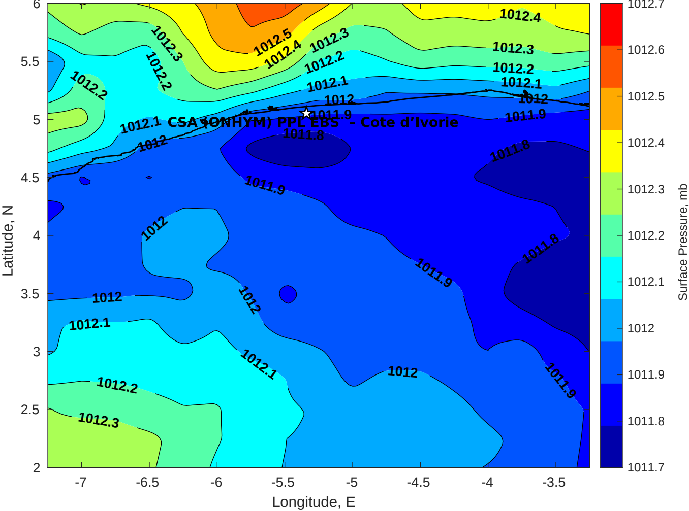
Surface Pressure (mb) for CSA (ONHYM) PPL EBS - Cote d'Ivoire at 16-Oct-2025 00:00:00
