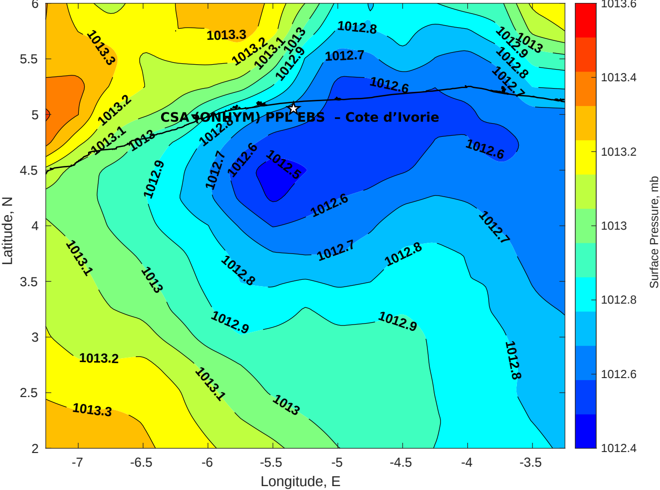
Surface Pressure (mb) for CSA (ONHYM) PPL EBS - Cote d'Ivoire at 18-Oct-2025 00:00:00
