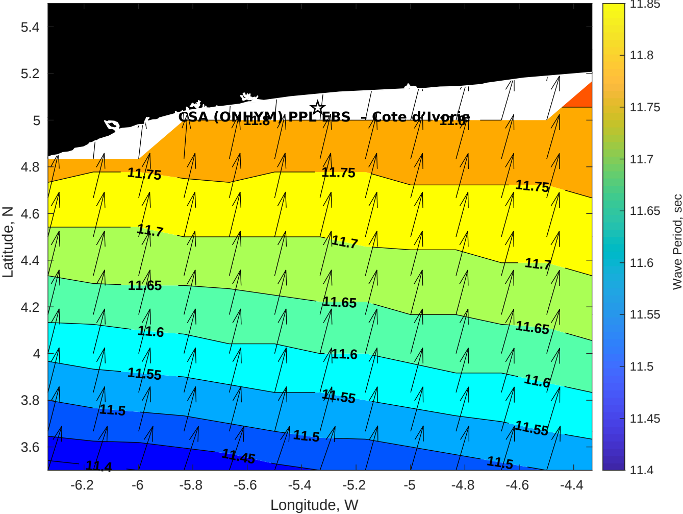
Wave Period (sec) for CSA (ONHYM) PPL EBS - Cote d'Ivoire at 16-Oct-2025 09:00:00
