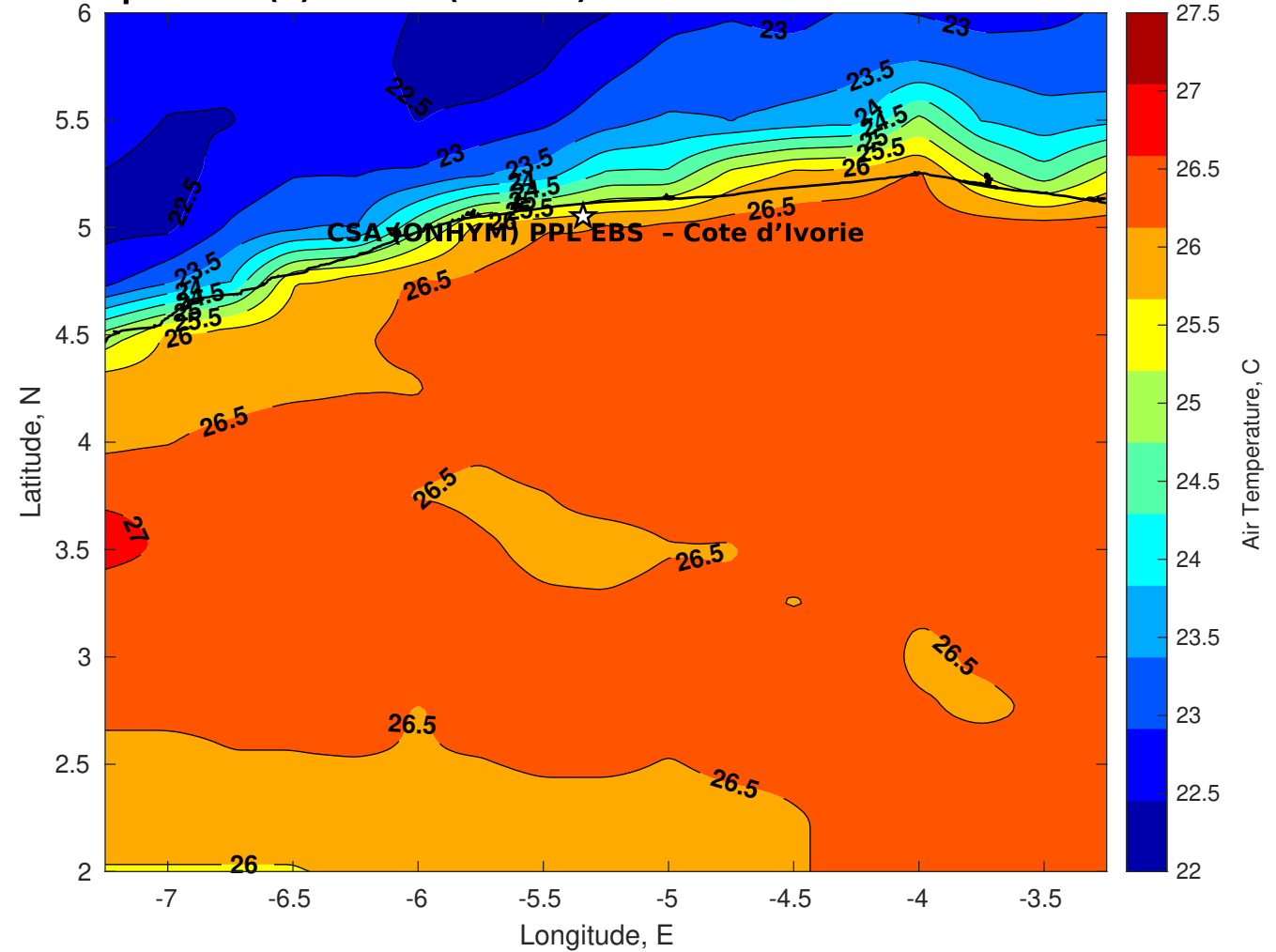
Air Temperature (C) for CSA (ONHYM) PPL EBS - Cote d'Ivoire at 16-Oct-2025
