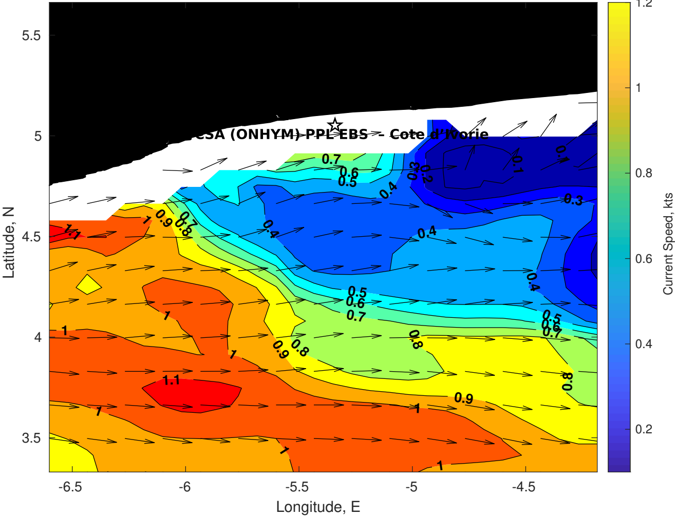
Surface Currents for CSA (ONHYM) PPL EBS - Cote d'Ivoire at 15-Oct-2025 00:00:00
