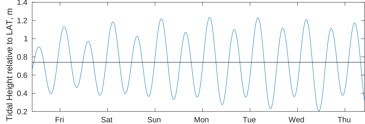
Tidal Currents and Heights for CSA (ONHYM) PPL EBS - Cote d'Ivoire at 20251016
