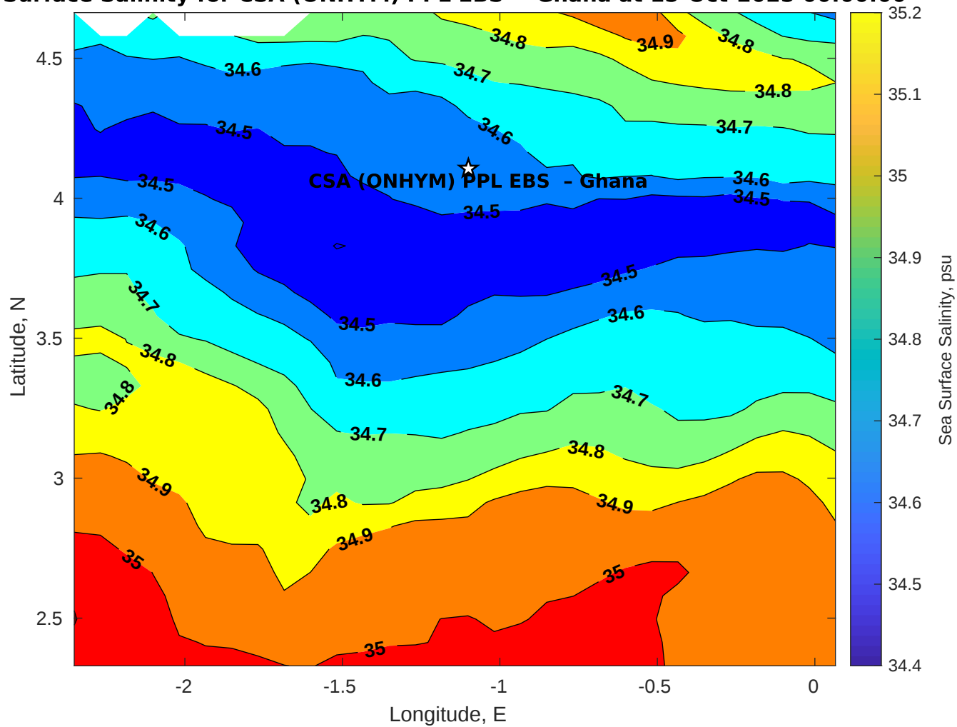
Surface Salinity for CSA (ONHYM) PPL EBS - Ghana at 15-Oct-2025 00:00:00
