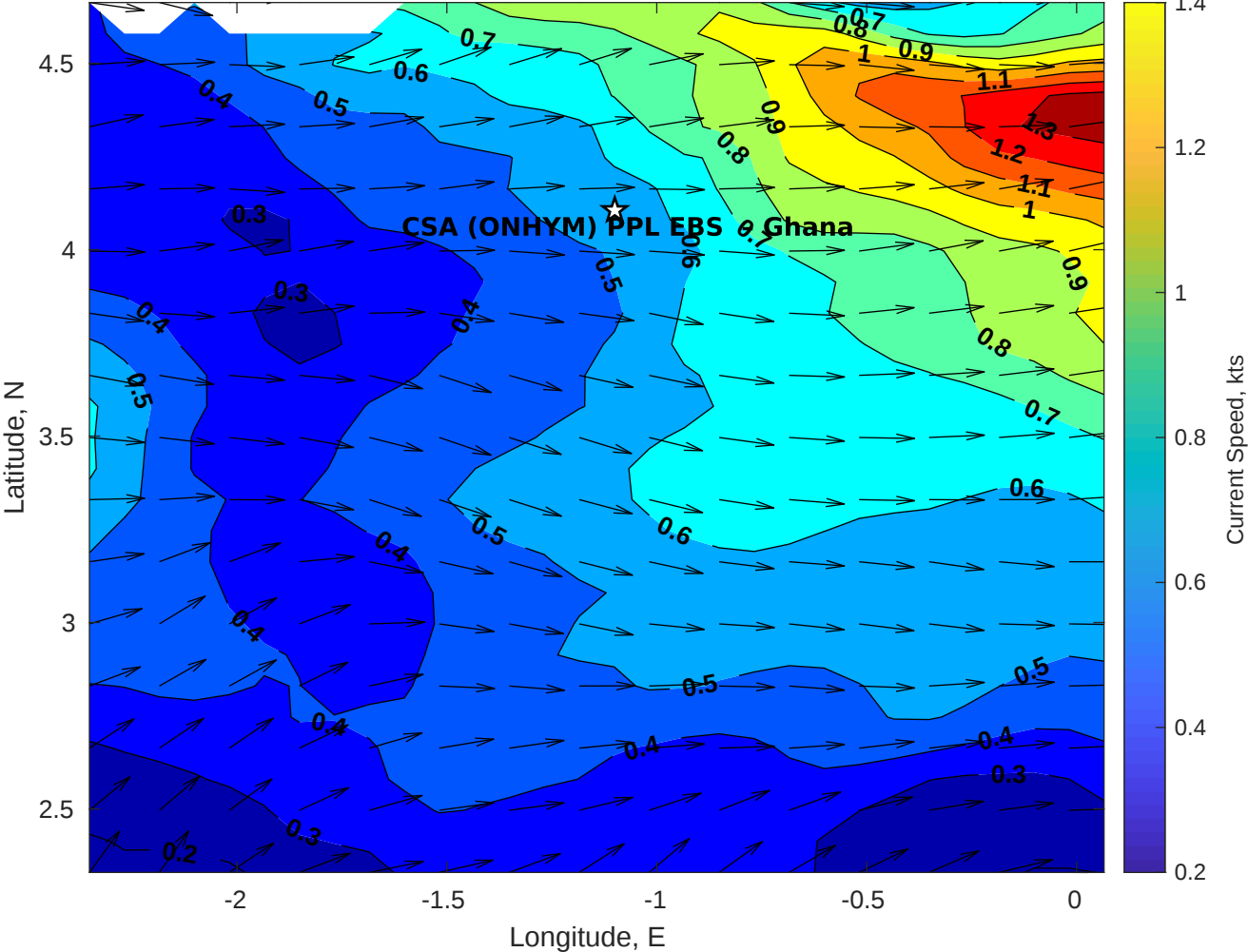
Surface Currents for CSA (ONHYM) PPL EBS - Ghana at 15-Oct-2025 00:00:00
