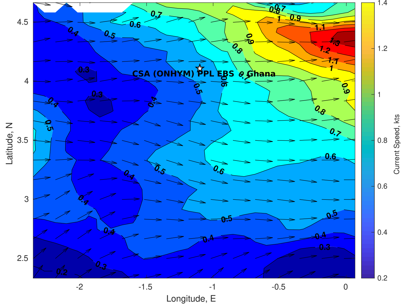
Surface Currents for CSA (ONHYM) PPL EBS - Ghana at 15-Oct-2025 00:00:00
