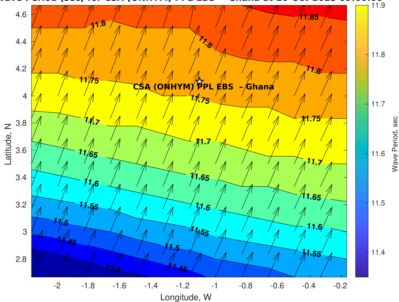
Wave Period (sec) for CSA (ONHYM) PPL EBS - Ghana at 16-Oct-2025 09:00:00
