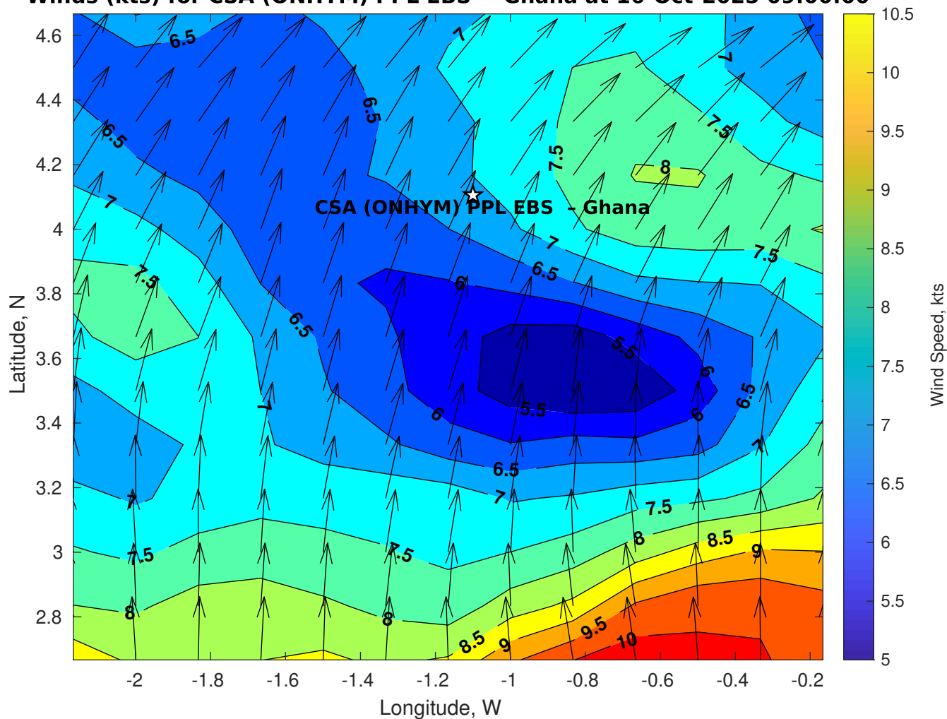
Winds (kts) for CSA (ONHYM) PPL EBS - Ghana at 16-Oct-2025 09:00:00
