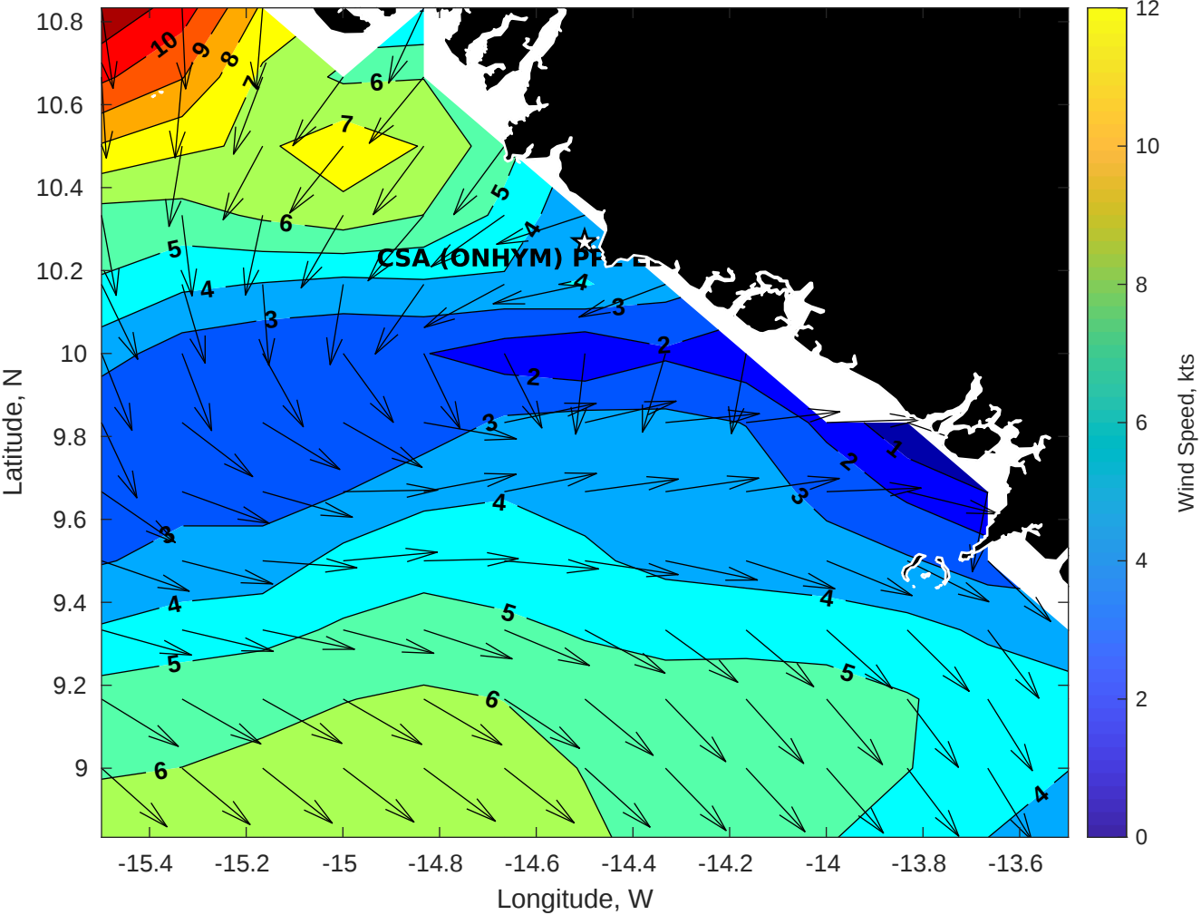
Winds (kts) for CSA (ONHYM) PPL EBS - Guinea at 16-Oct-2025 09:00:00
