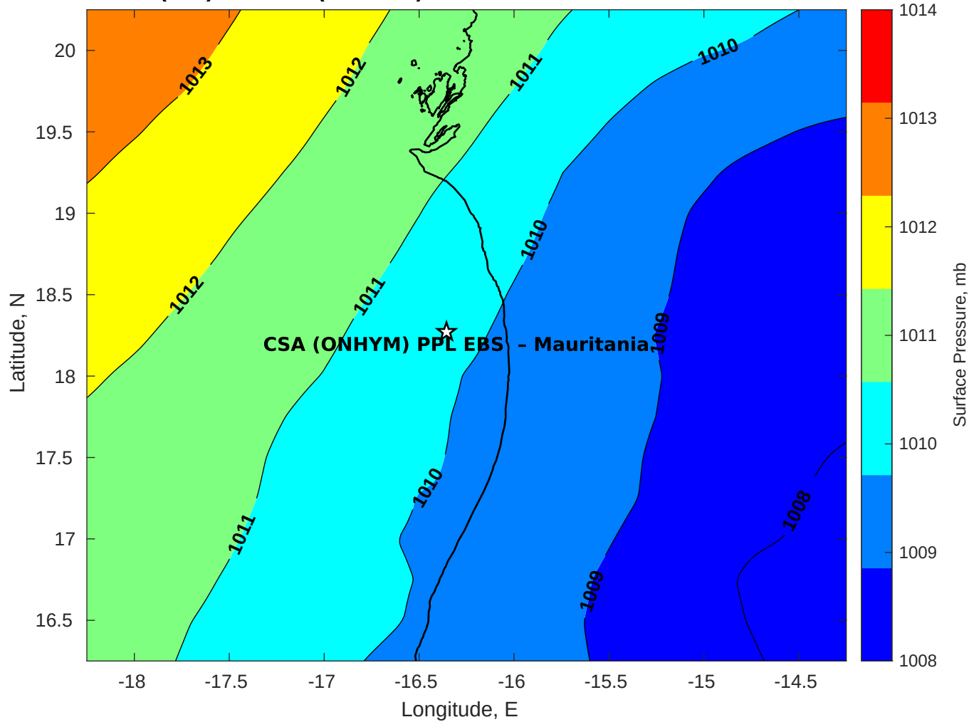
Surface Pressure (mb) for CSA (ONHYM) PPL EBS - Mauritania at 17-Oct-2025 00:00:00
