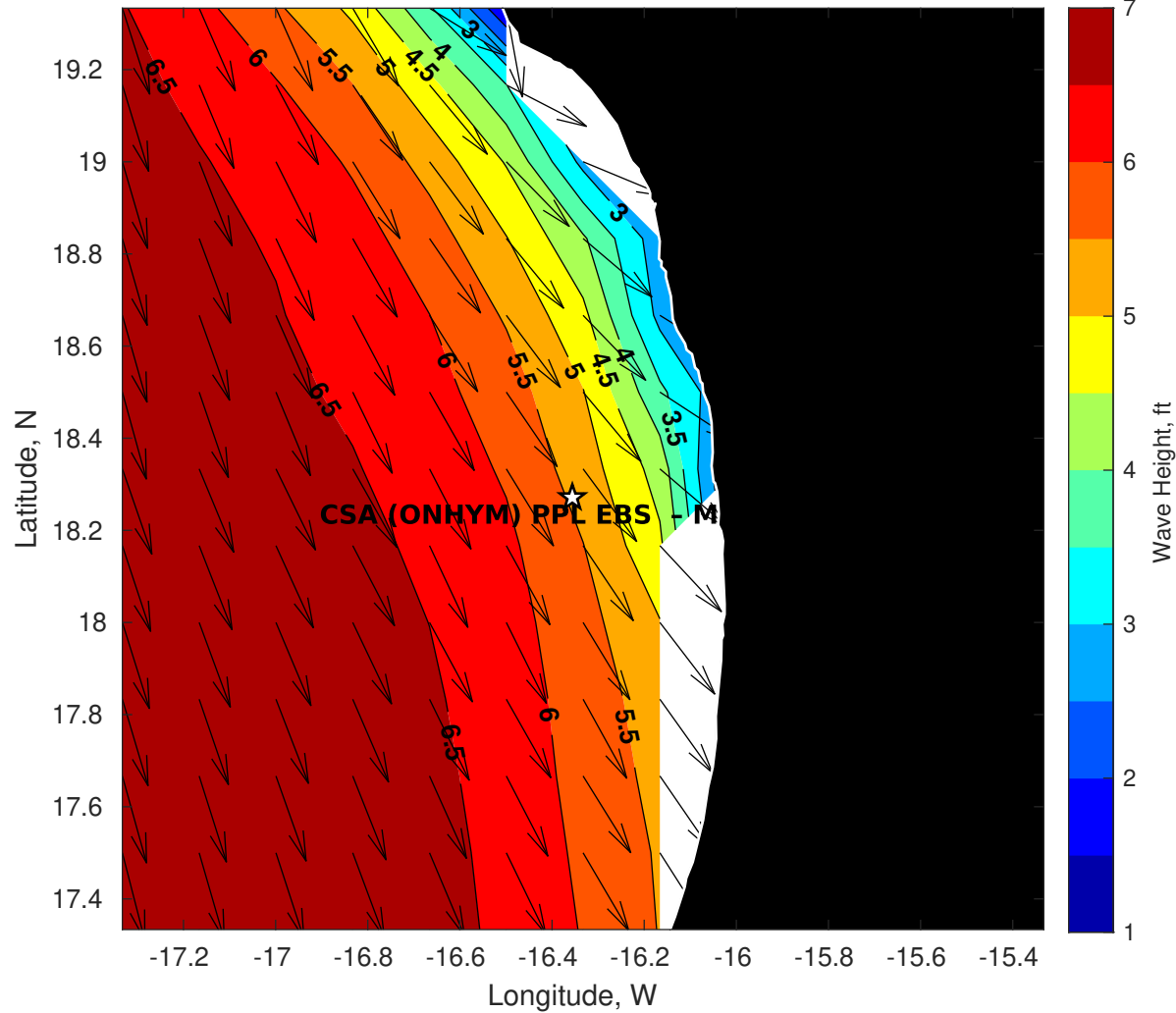
Wave Height (ft) for CSA (ONHYM) PPL EBS - Mauritania at 16-Oct-2025 09:00:00
