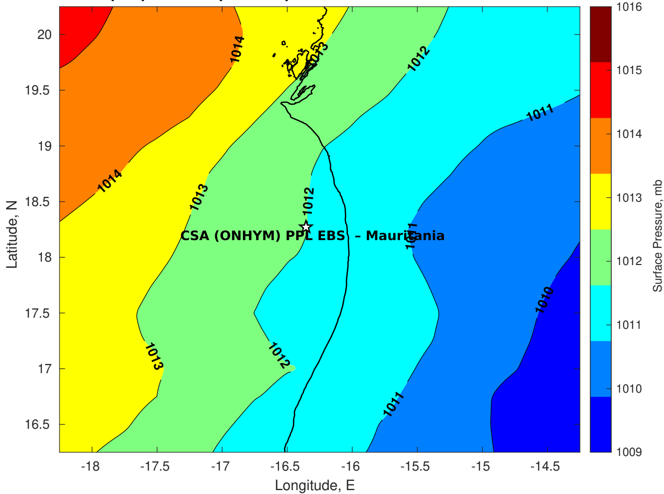
Surface Pressure (mb) for CSA (ONHYM) PPL EBS - Mauritania at 16-Oct-2025 00:00:00
