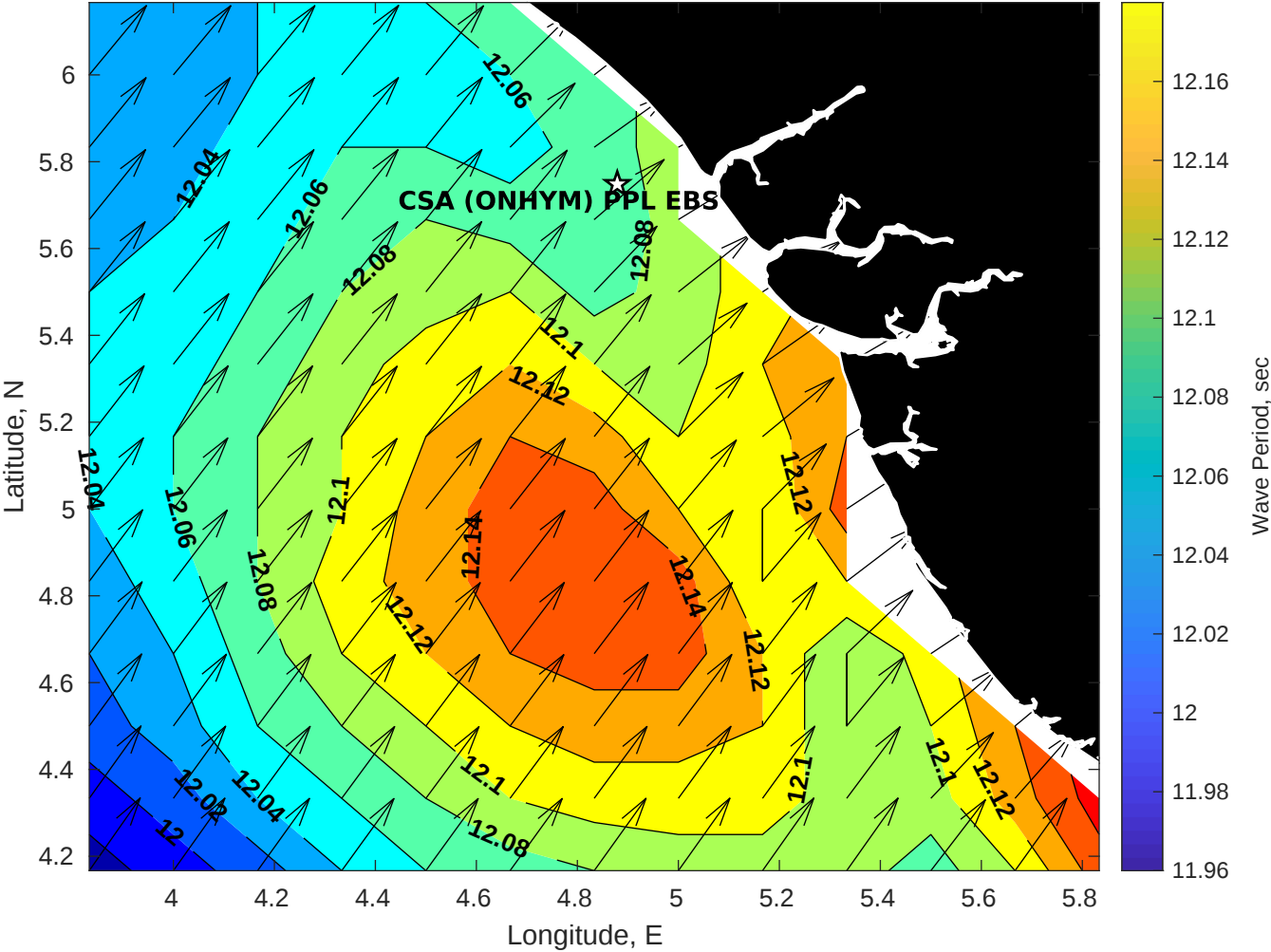
Wave Period (sec) for CSA (ONHYM) PPL EBS - Nigeria at 16-Oct-2025 09:00:00
